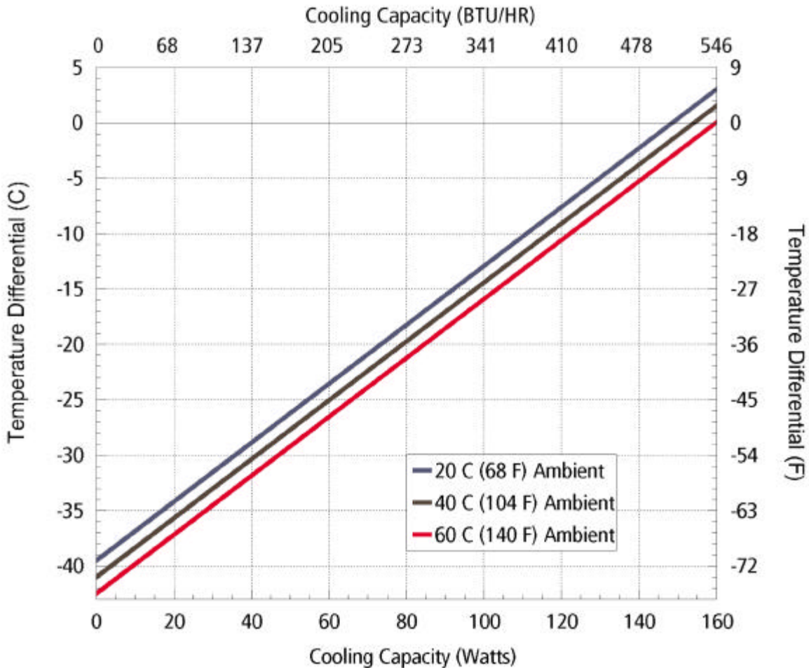
AHP-1200FF/XE/X PERFORMANCE CURVE
