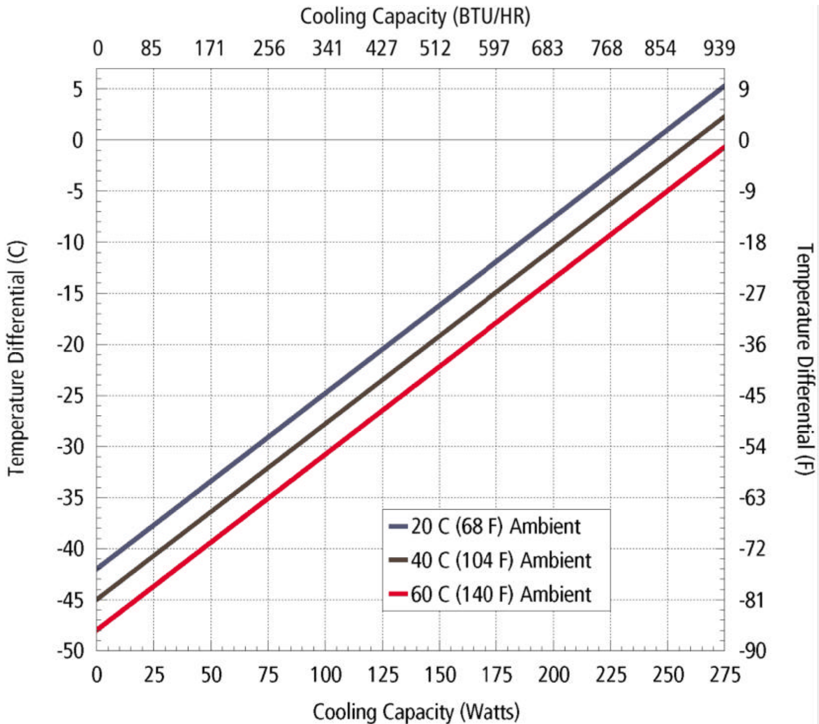
AHP-1200CP Performance curve
