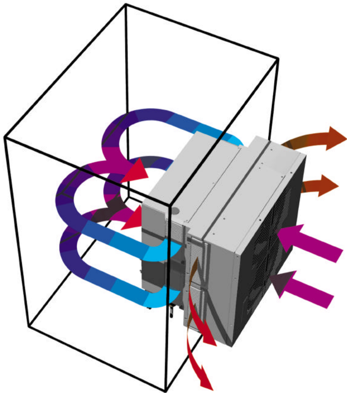
AHP-1400 Air flow pattern
