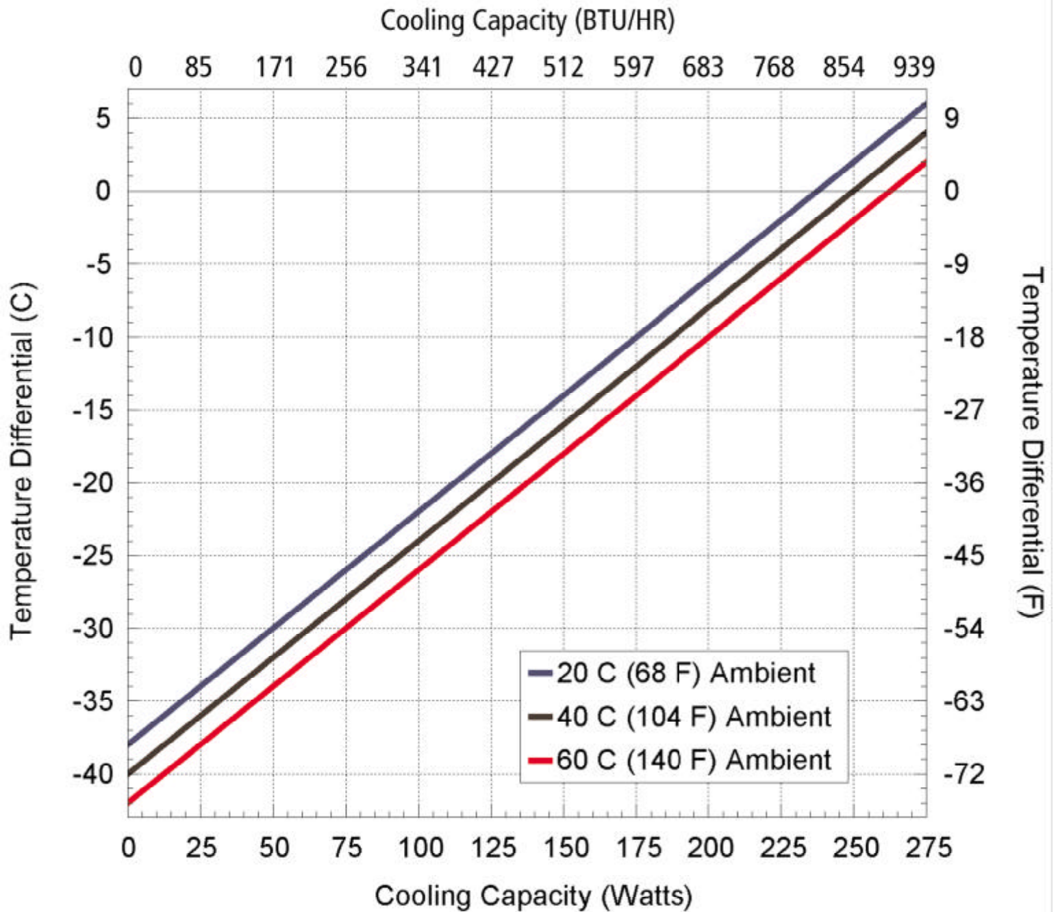
AHP-1400 Performance curve
