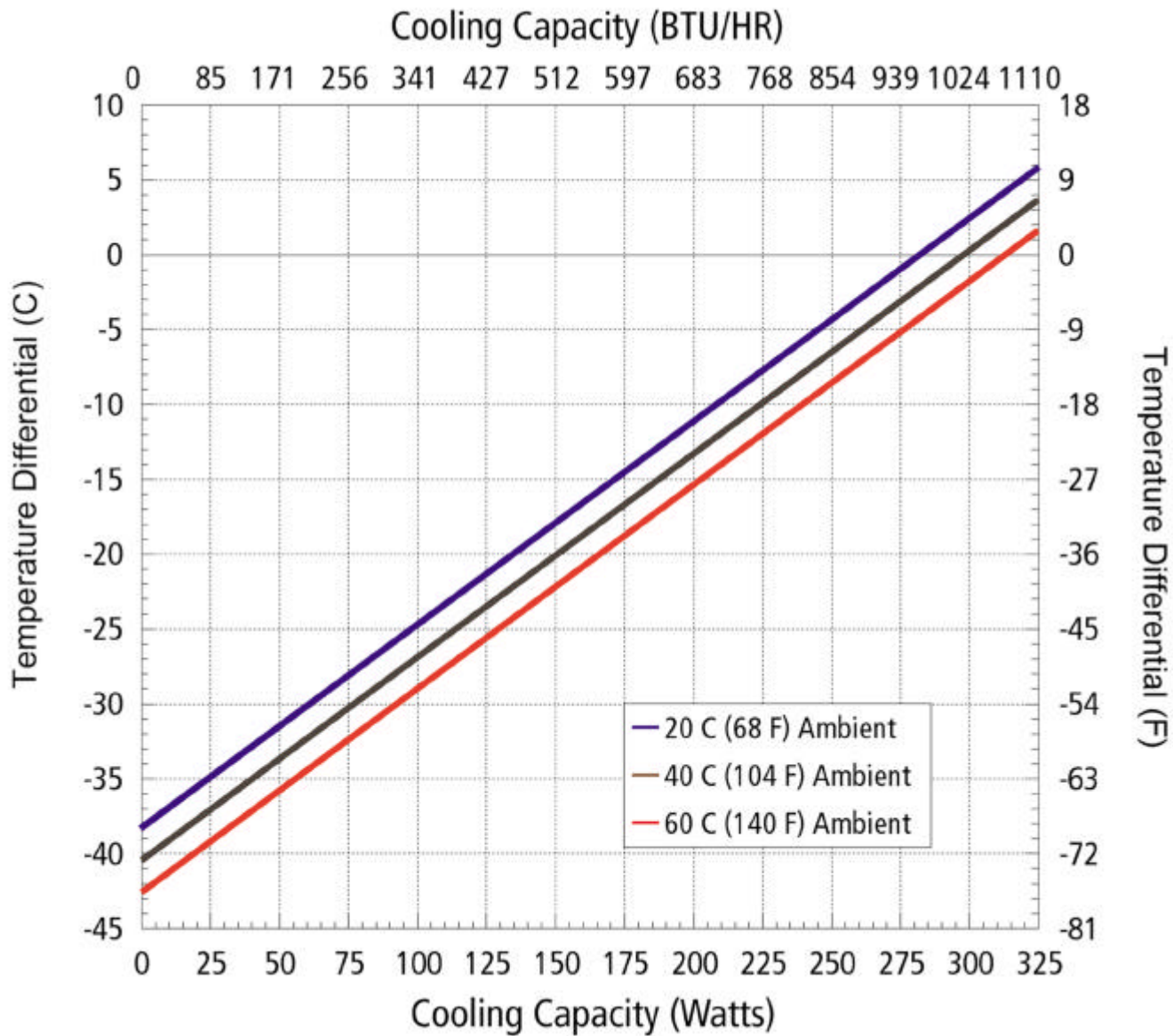
AHP-1501/1501XE Performance curve
