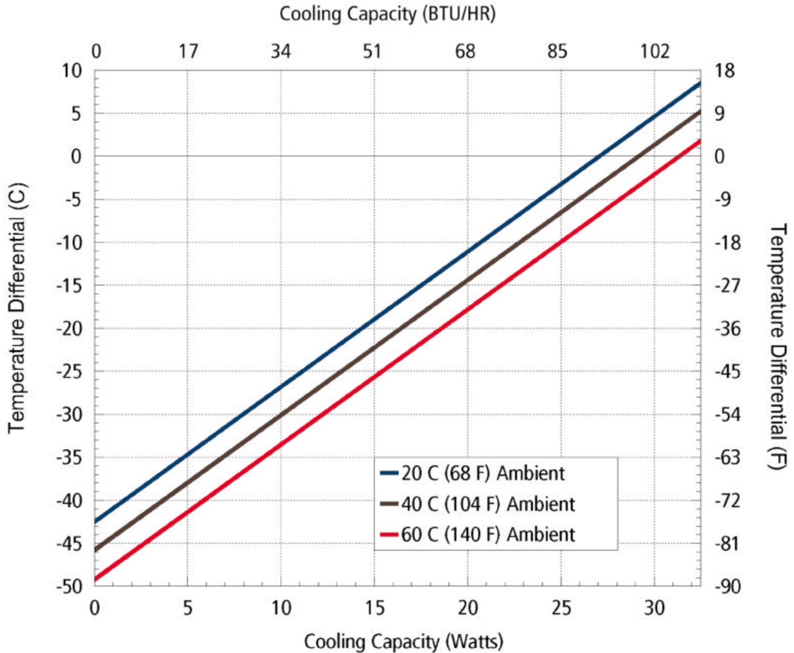
AHP-150FF/150XE Performance curve
