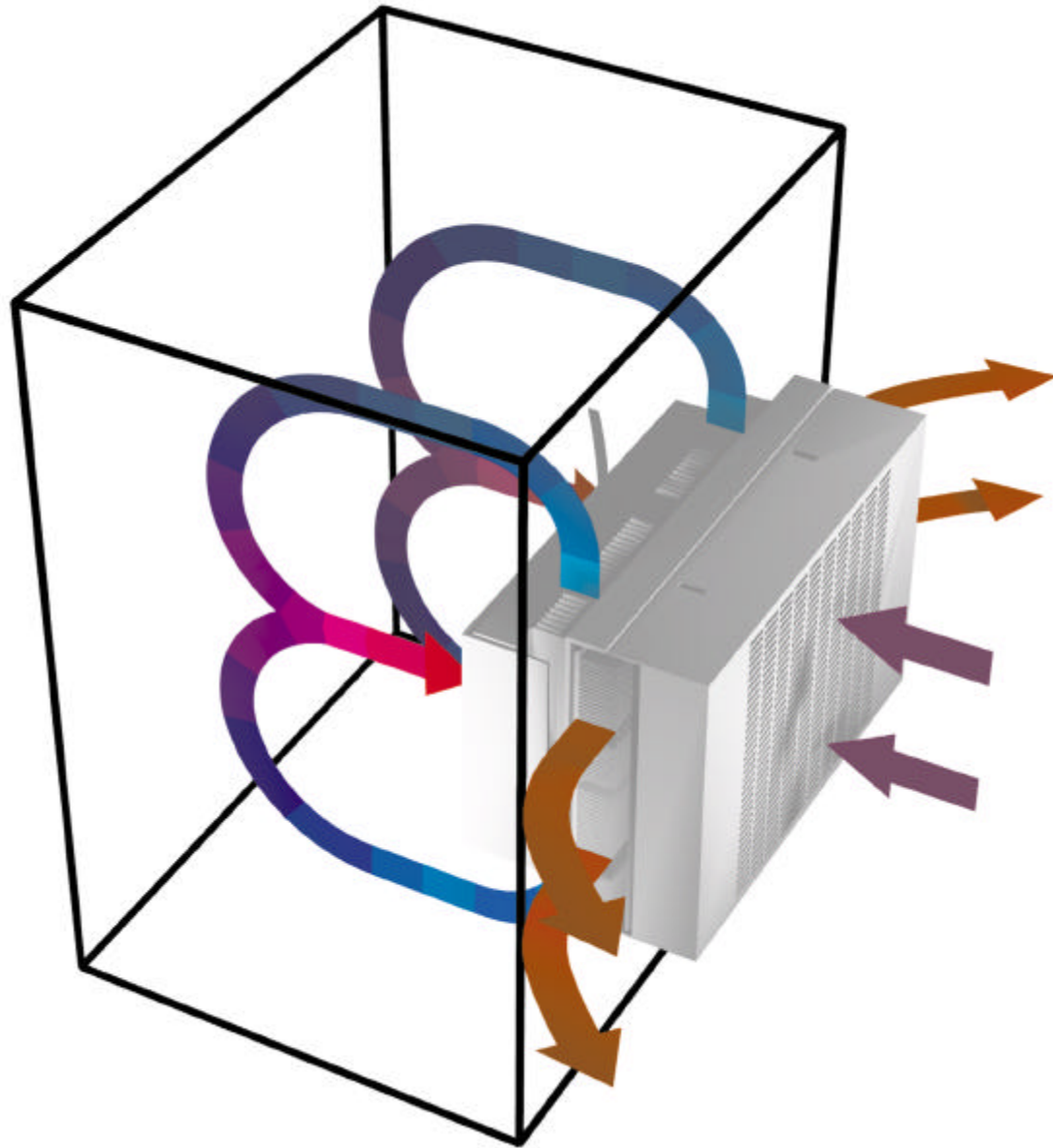
AHP-1800/1801/1802 Series air flow pattern
