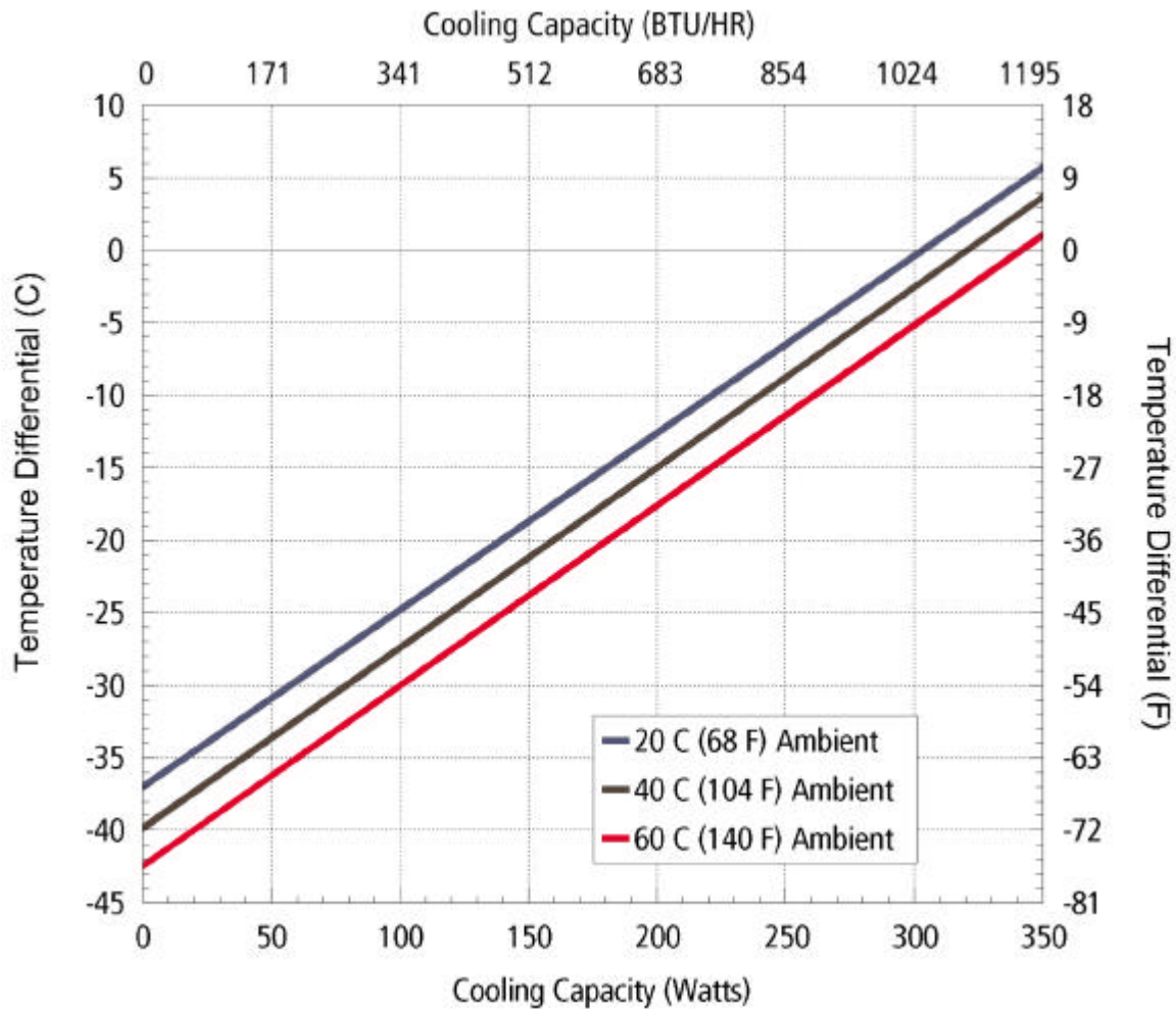
AHP-1800/1801/1802 Series performance curve
