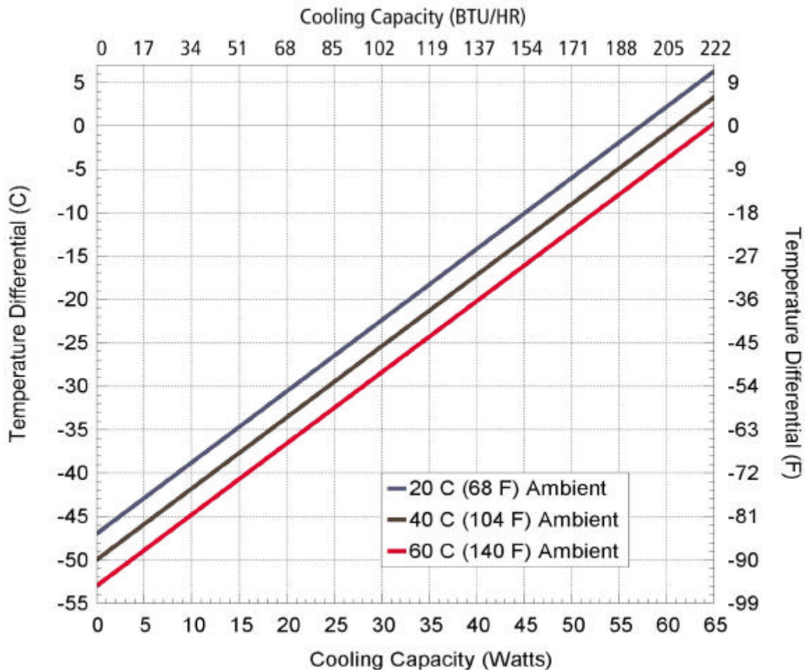
AHP-300FF/XE/X Performance Curve
