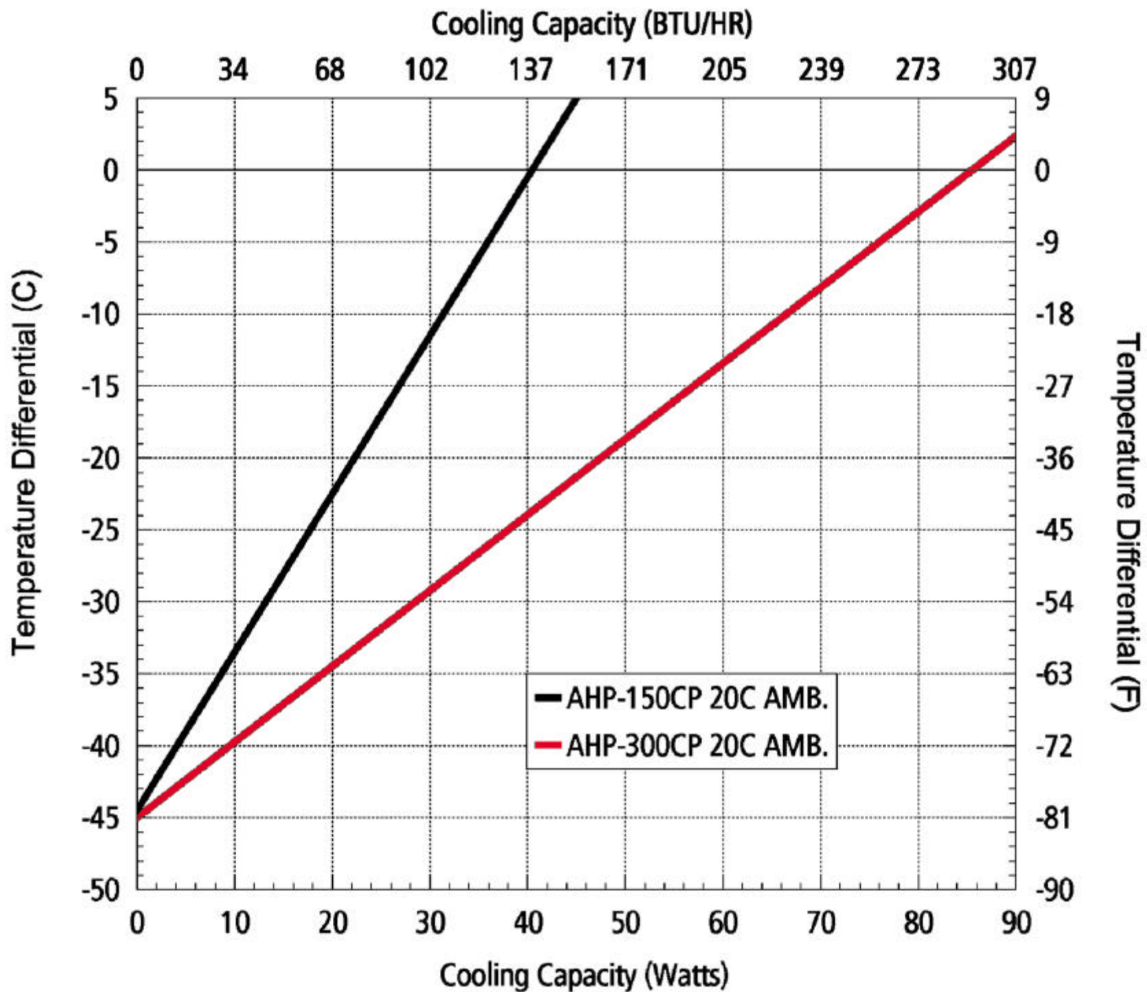
AHP-300CP / AHP-150CP Performance curve
