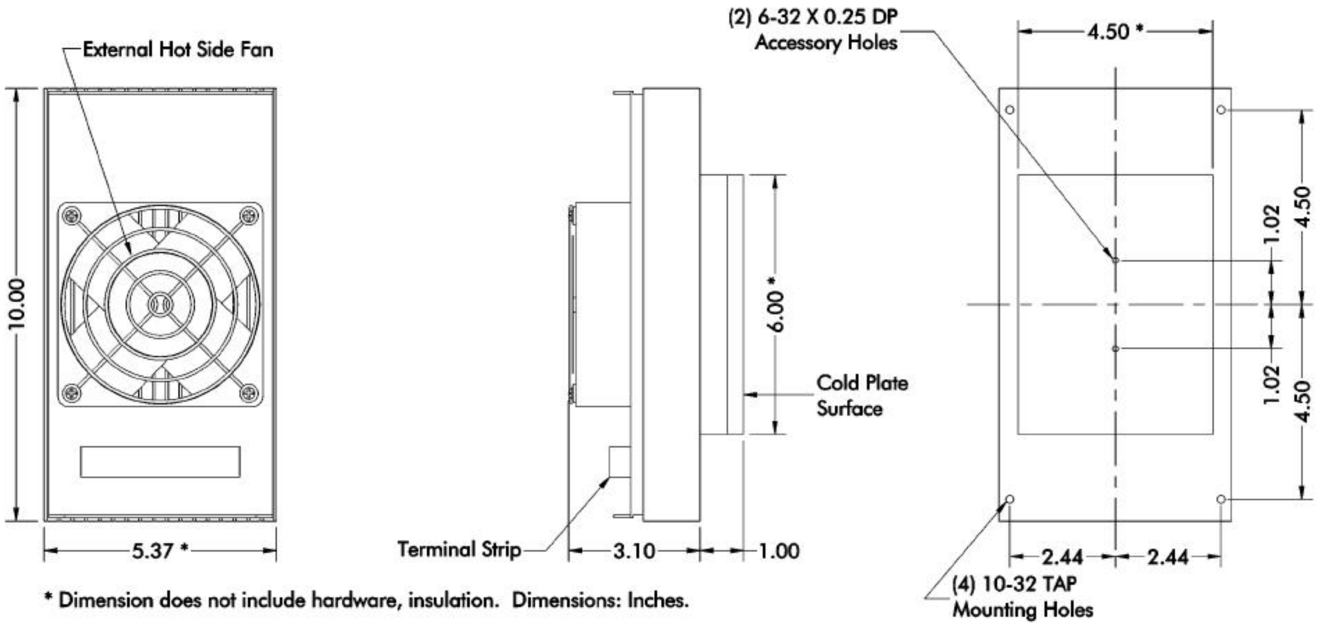
AHP-300CP Dimensional drawing
