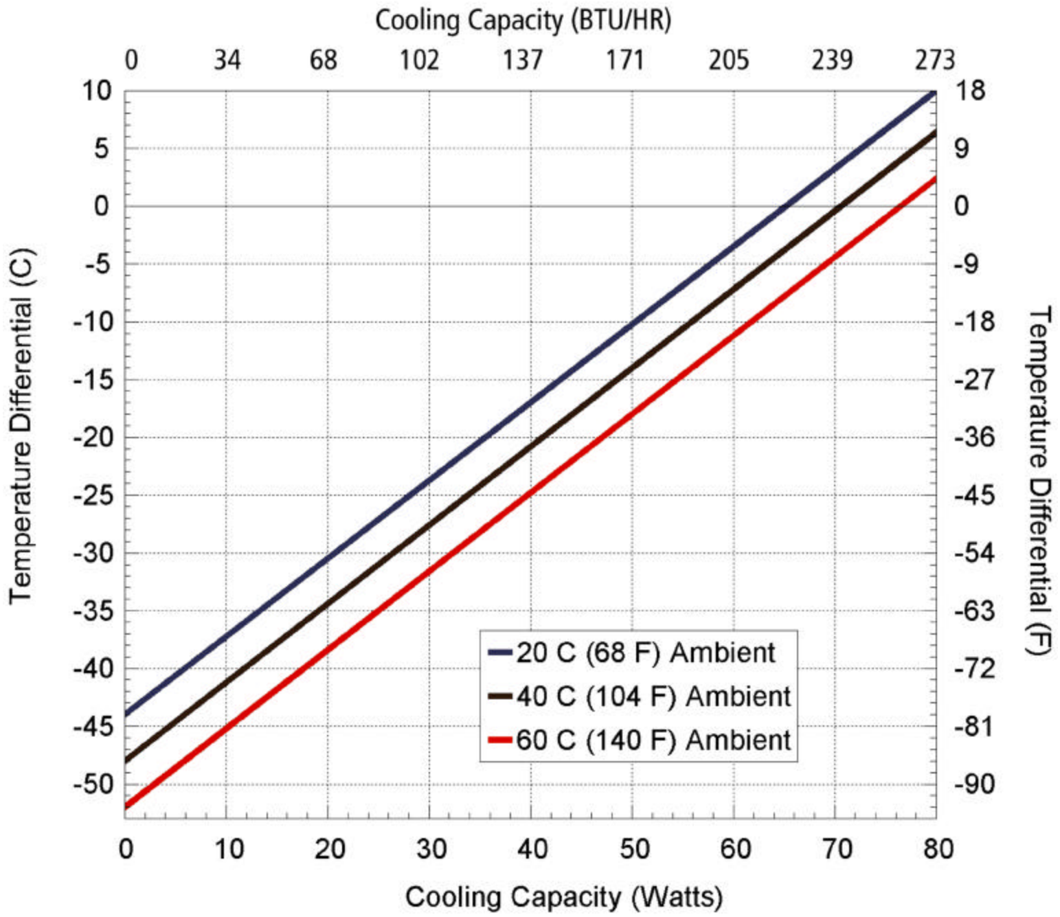
AHP-301CP Performance curve
