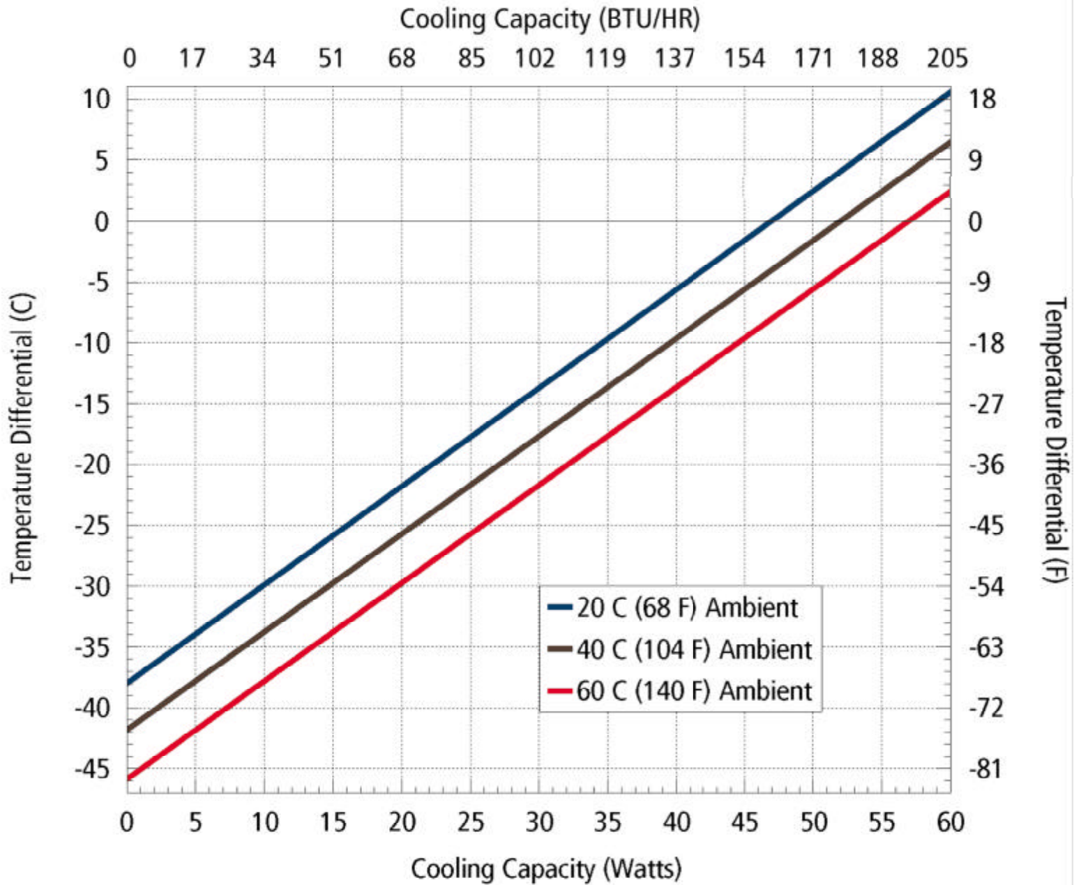
AHP-301FF Performance curve
