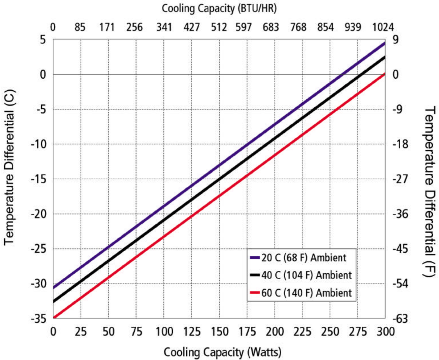
FHP-1501 / 1501XE Performance curve
