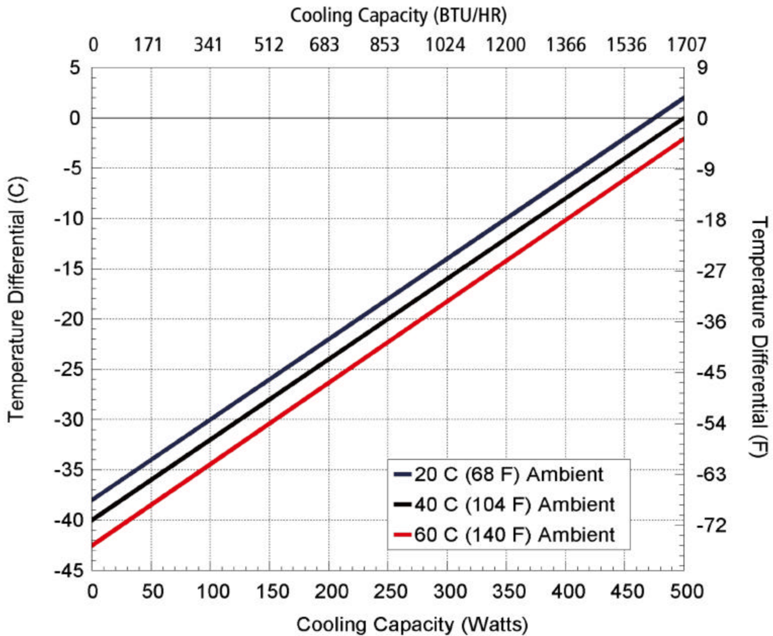
FHP-2850 / 2852 Performance curve
