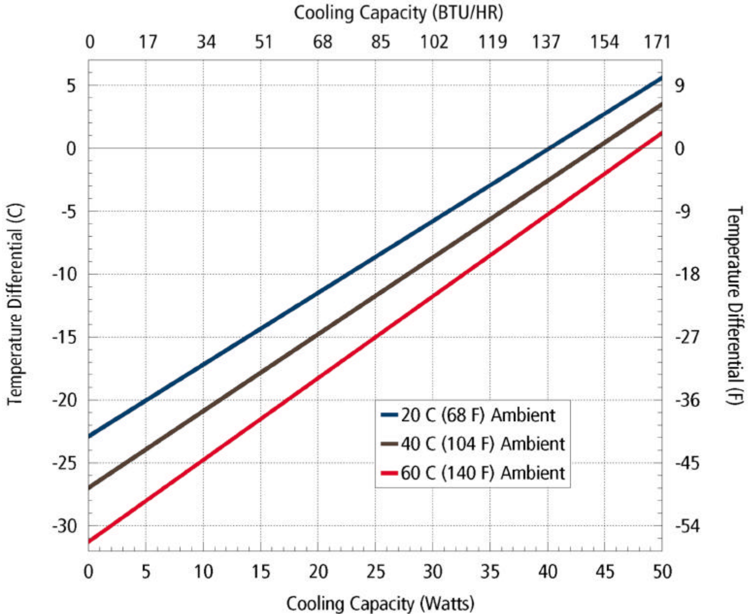
FHP-450XE / 452XE Performance curve
