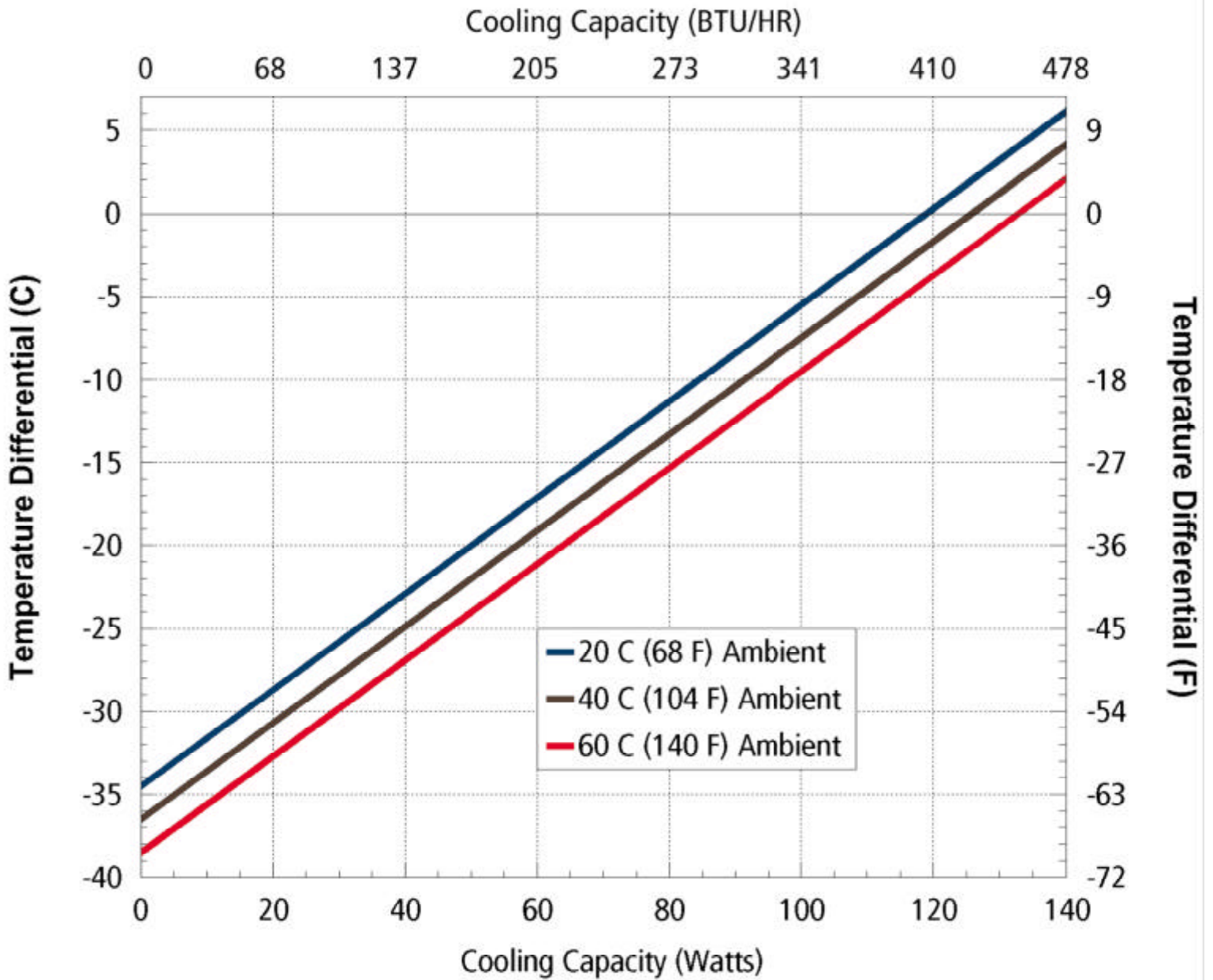
FHP-750 / 752 / XE Performance curve
