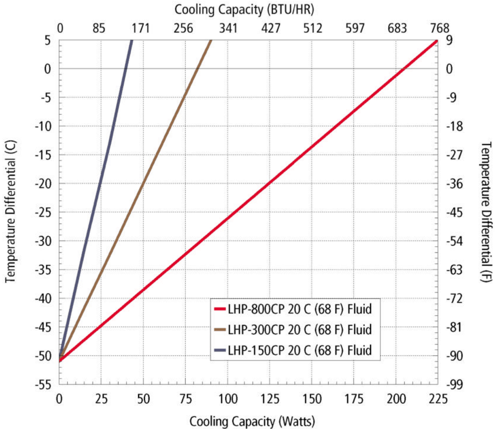
LHP-800CP/300CP/150CP Performance curve
