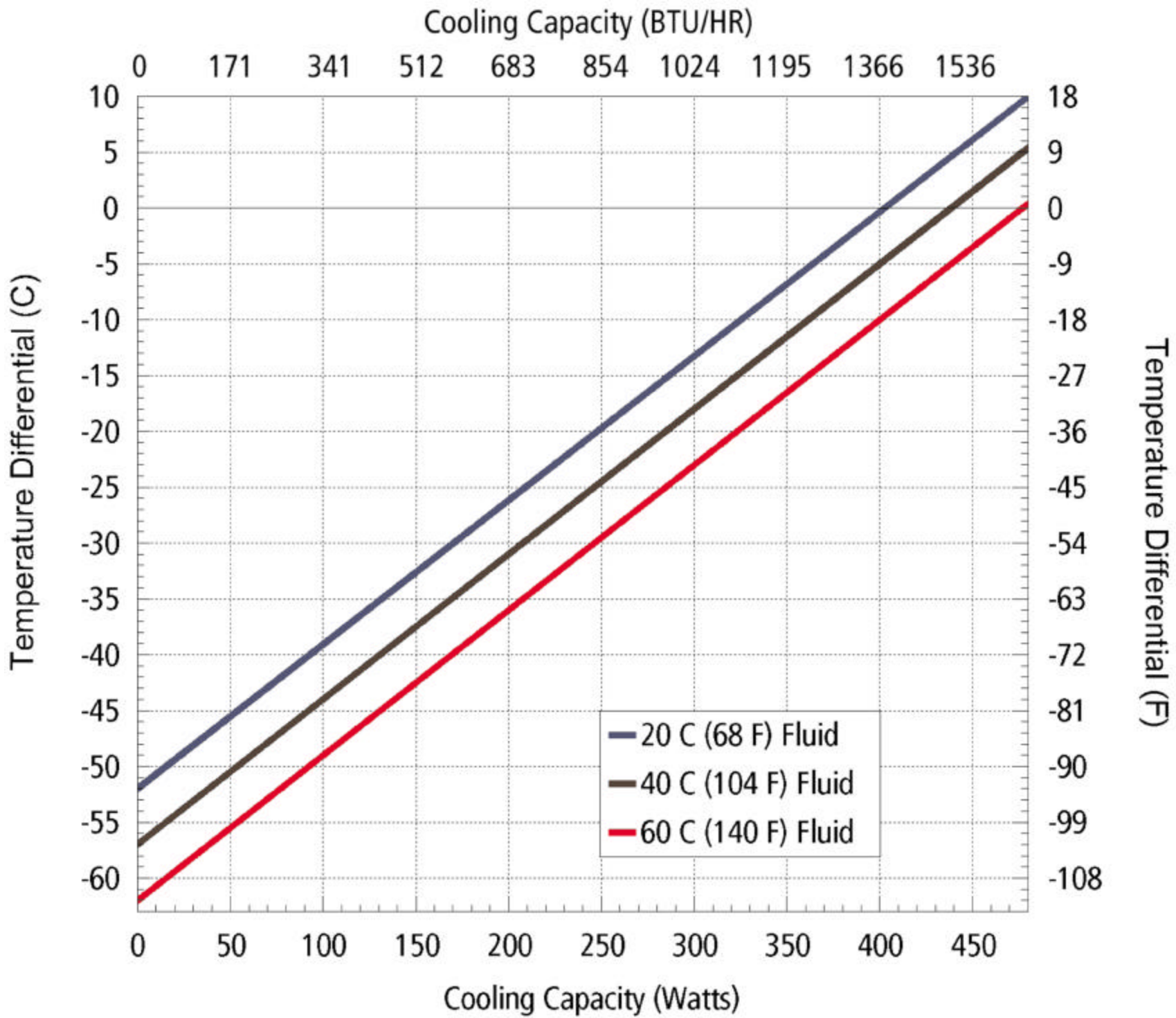
LHP-1700CP Performance curve
