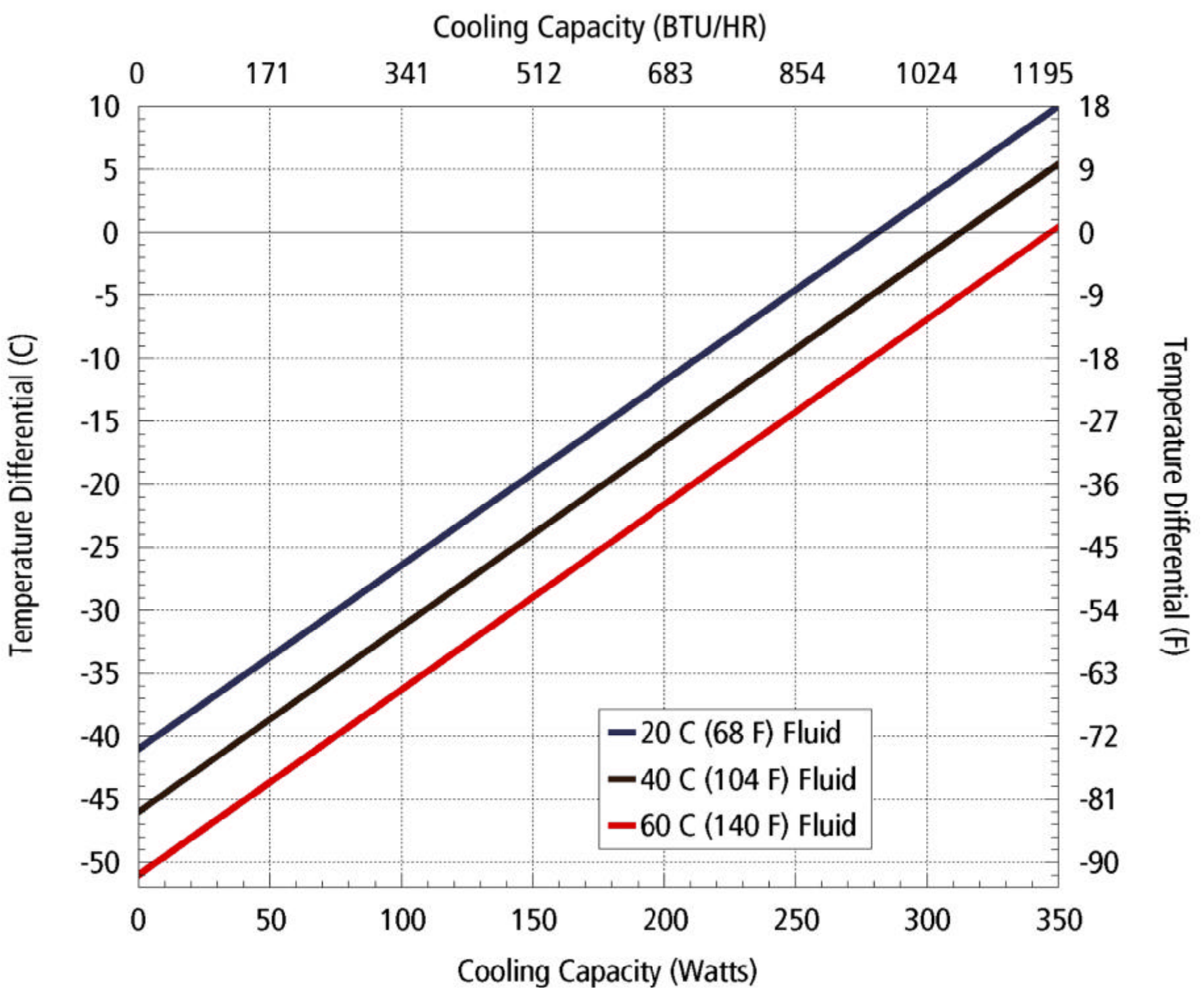
LHP-1700FF Performance curve
