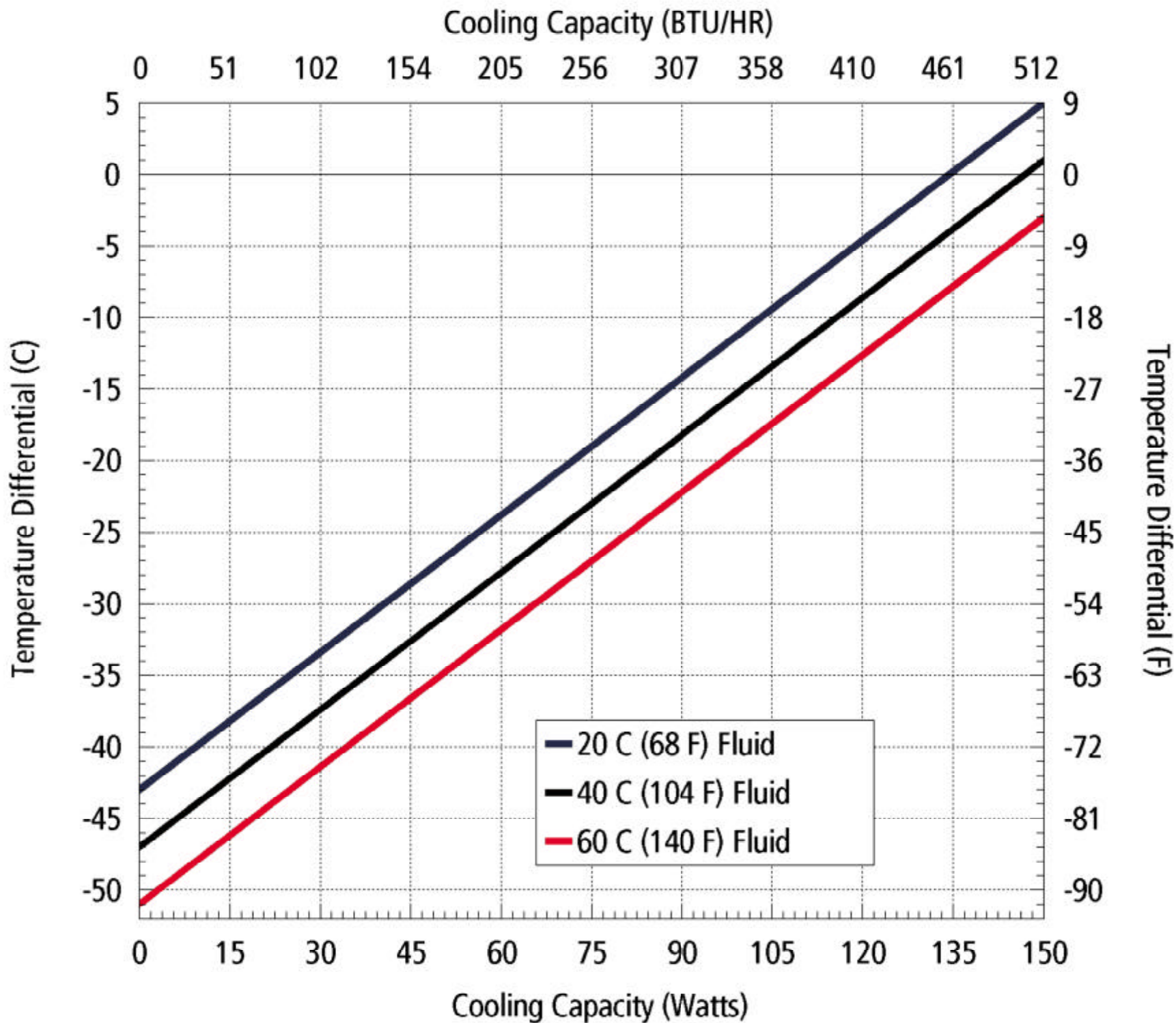
LHP-800FF Performance curve
