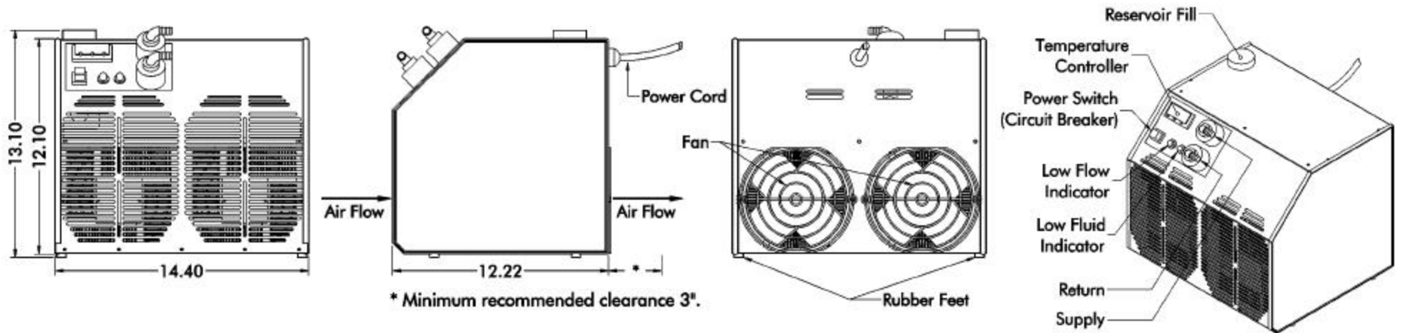
TLC-1400 Dimensional drawing
