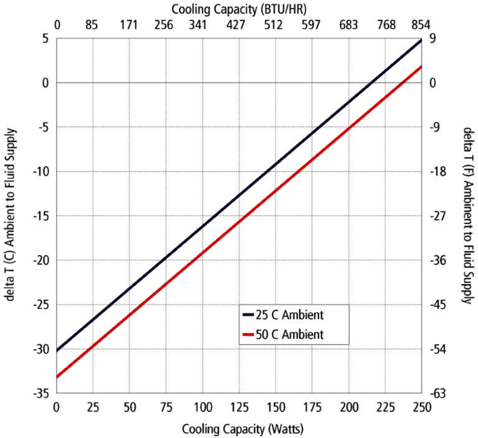
TLC-700/702 Performance curve
