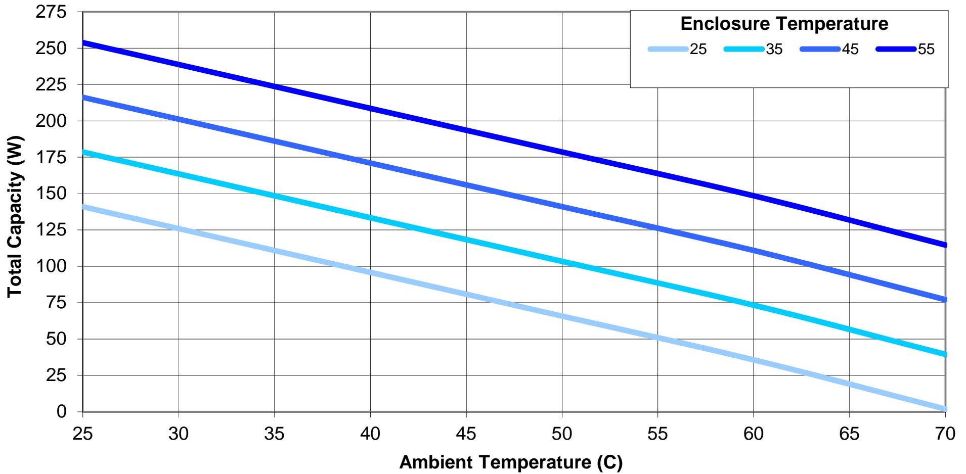
AHP-1200 Cooling for various Enclosure Temperatures
