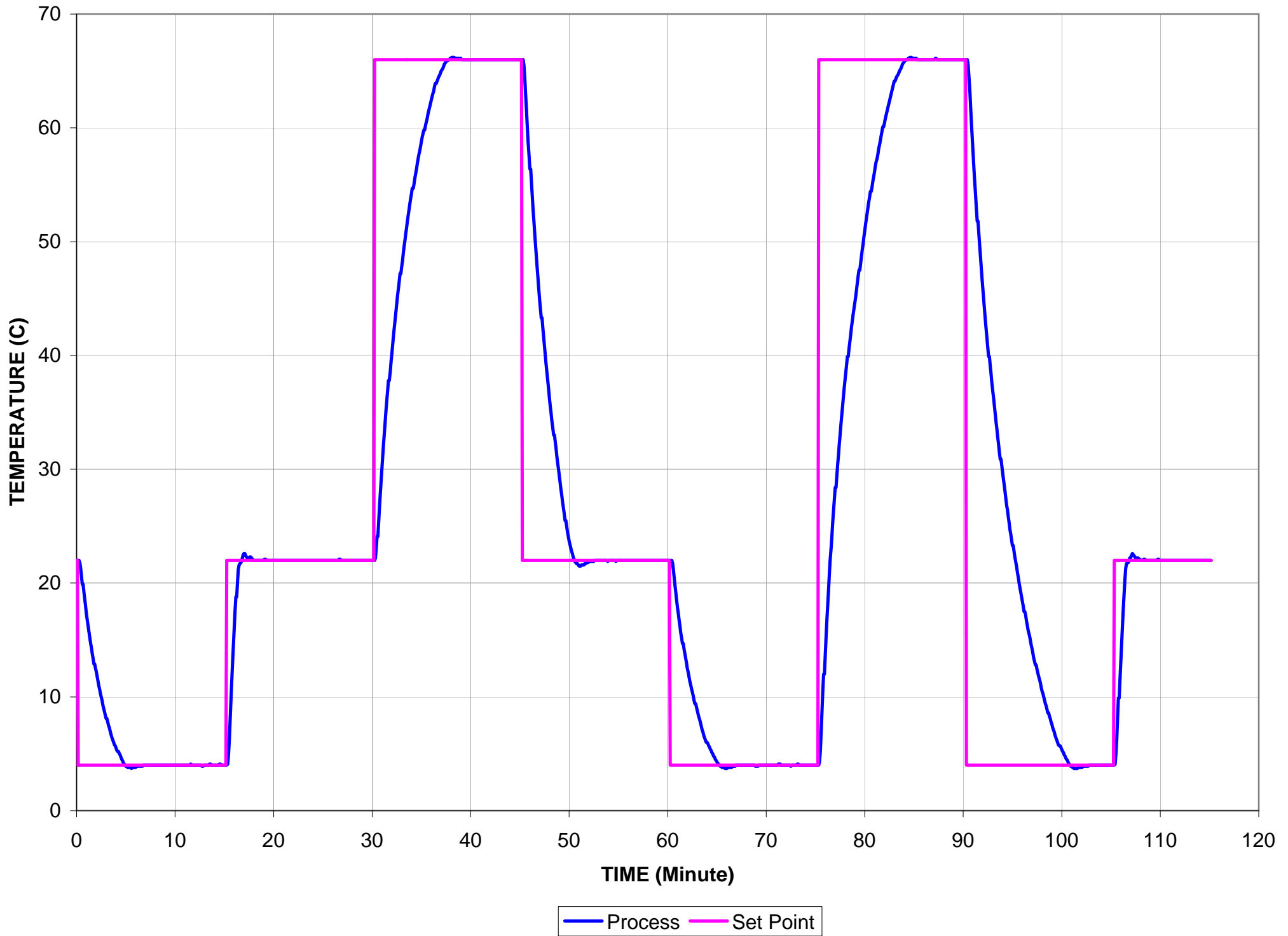
AHP-1200DCP Fan speed @ 50% Uncovered
