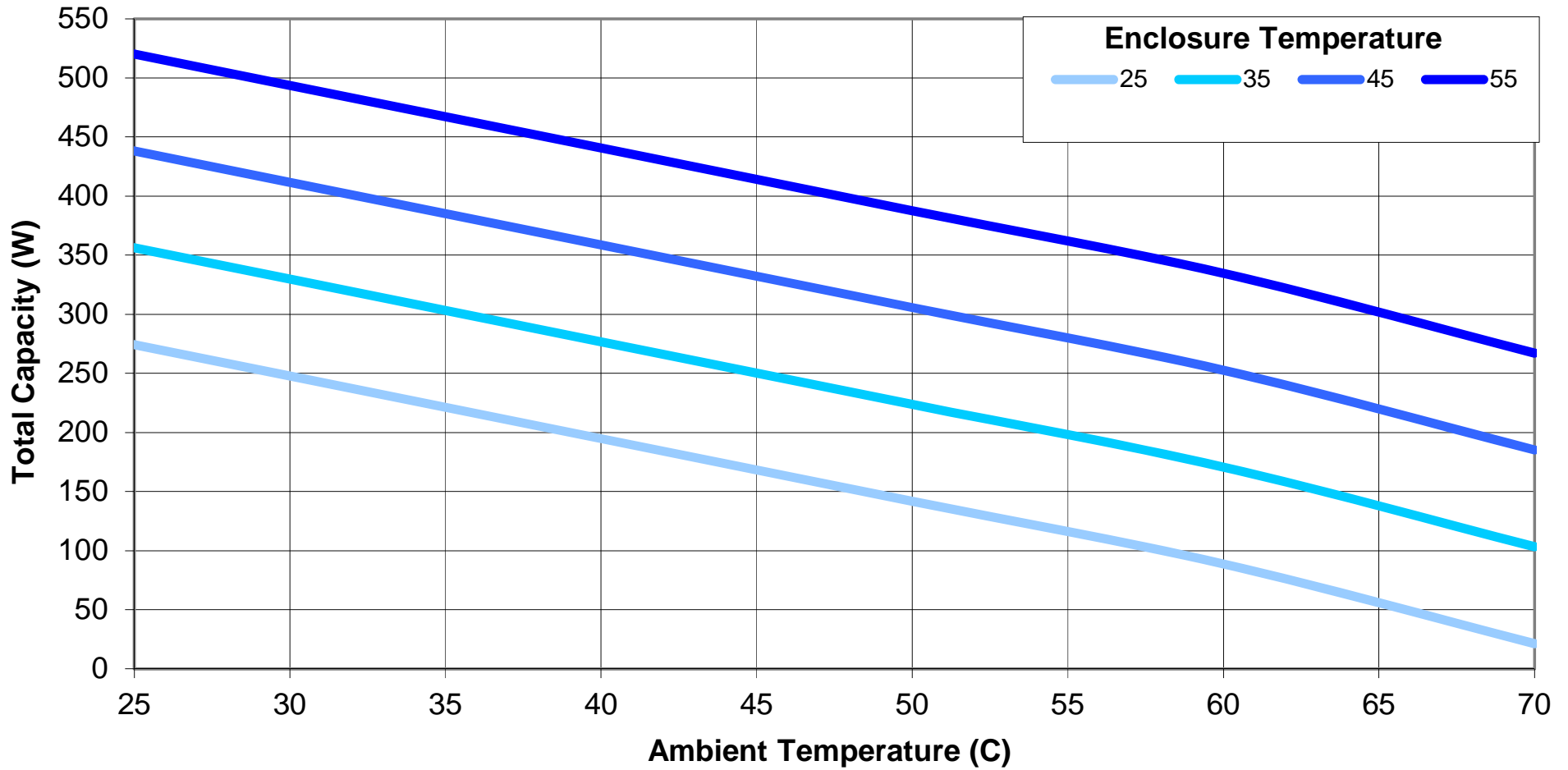
AHP-1801 Cooling for various Enclosure Temperatures
