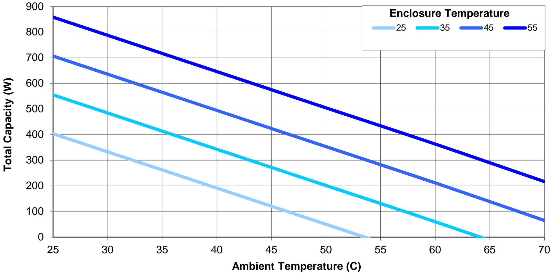
AHP-2250DC Cooling for various Enclosure Temperatures
