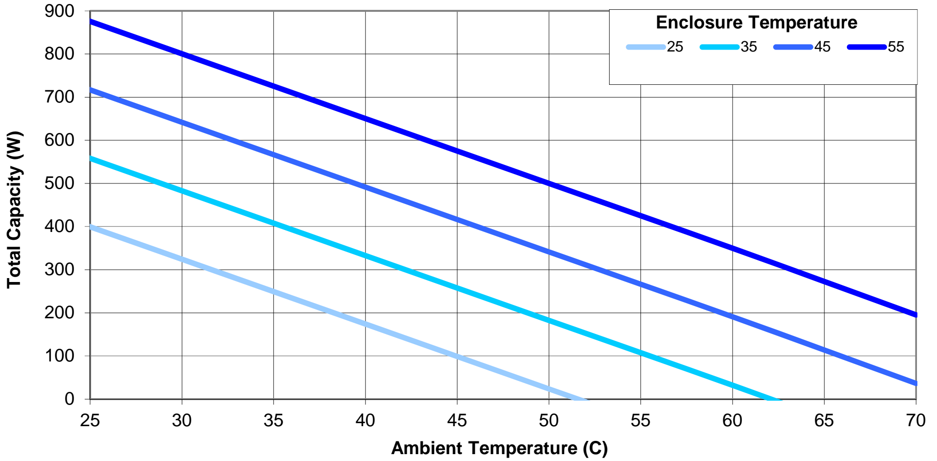
AHP-2250 HiE Cooling for various Enclosure Temperatures
