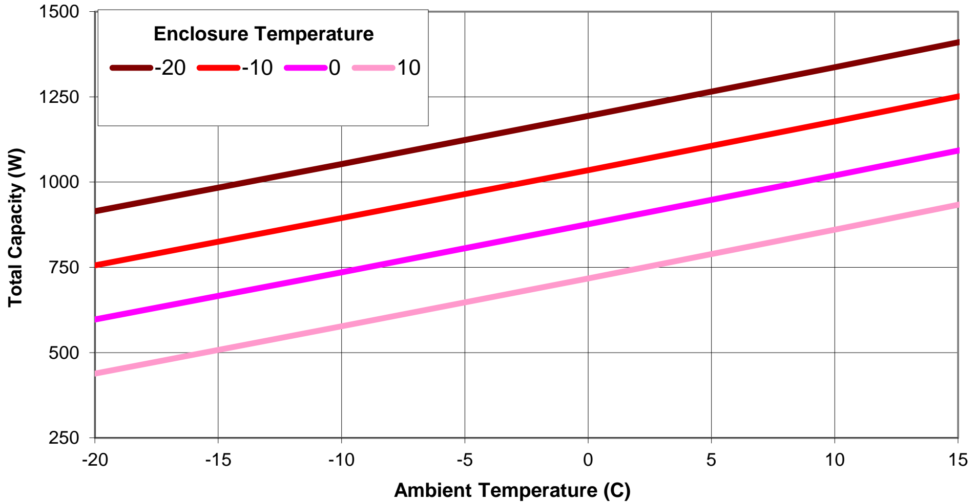
AHP-2250 HiE Heat Mode Cap for various Enclosure Temperatures
