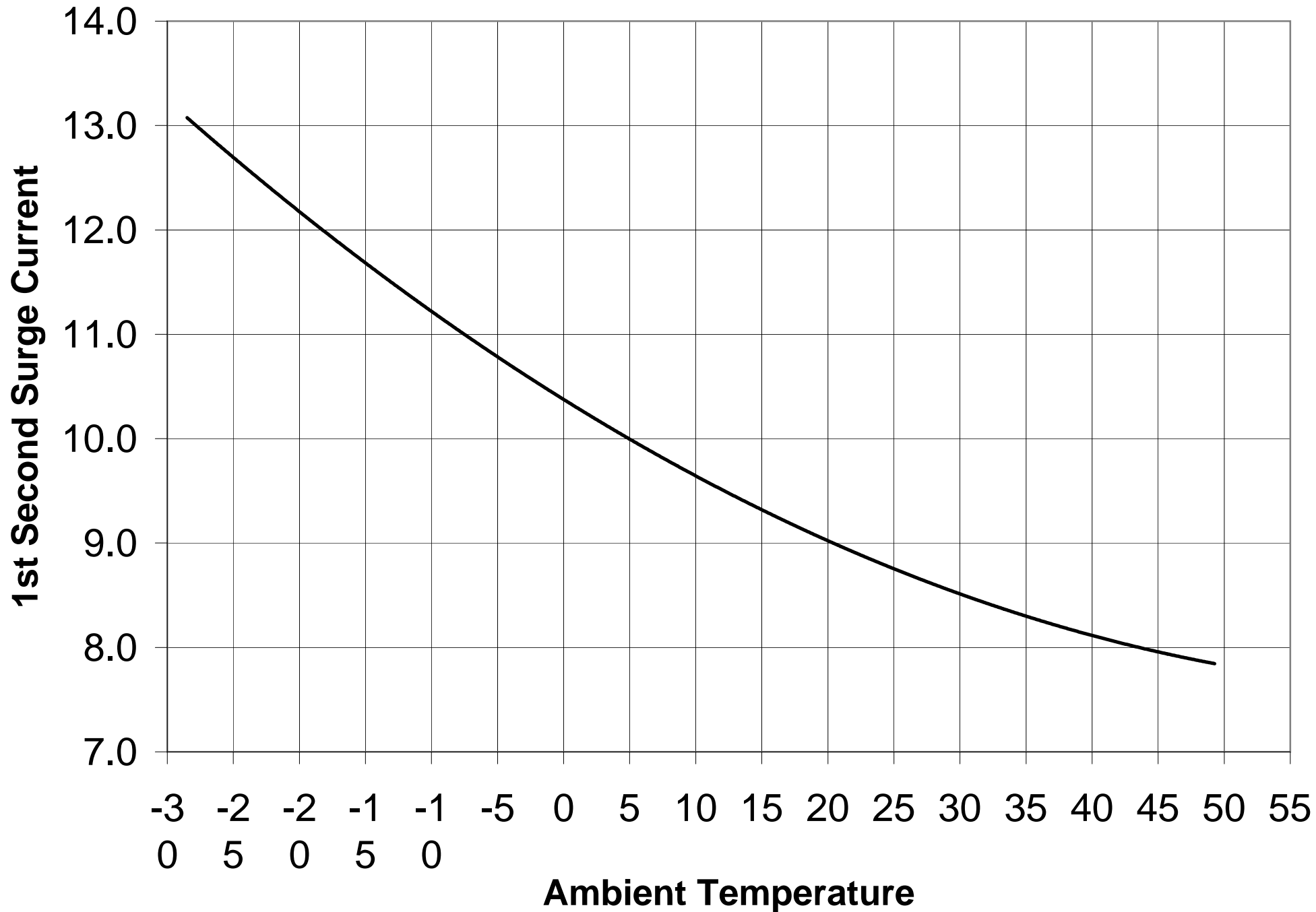
Start Up Current, AHP-2252 Hi Cap, by ambient temperature
