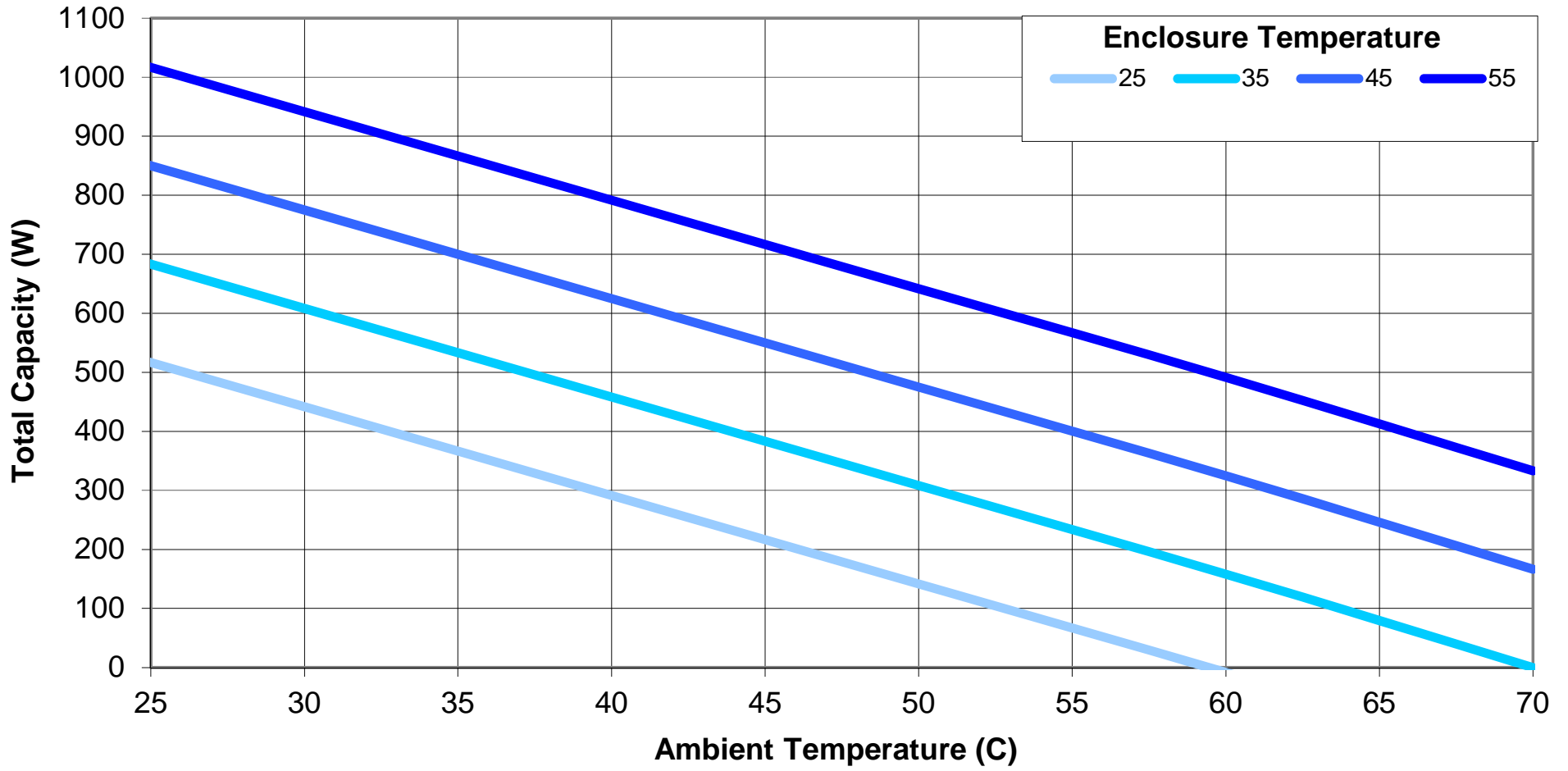
AHP-2259 HiCap Cooling for various Enclosure Temperatures
