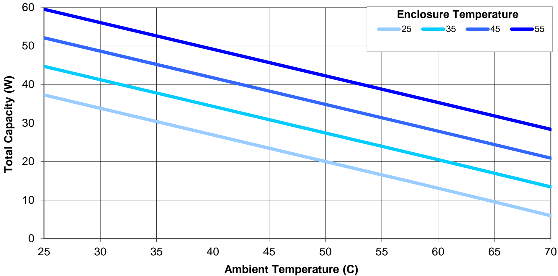
AHP-250 Cooling for various Enclosure Temperatures
