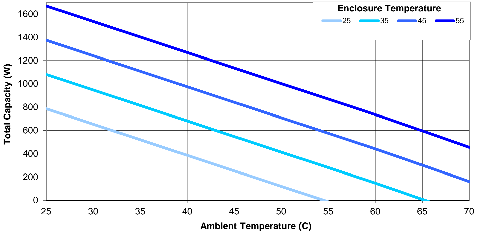
AHP-4252 HiE Cooling for various Enclosure Temperatures
