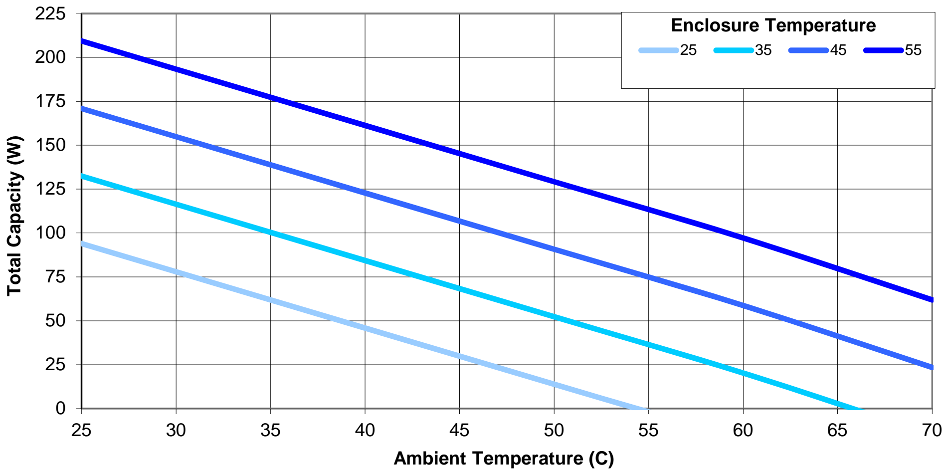
AHP-451 Cooling for various Enclosure Temperatures
