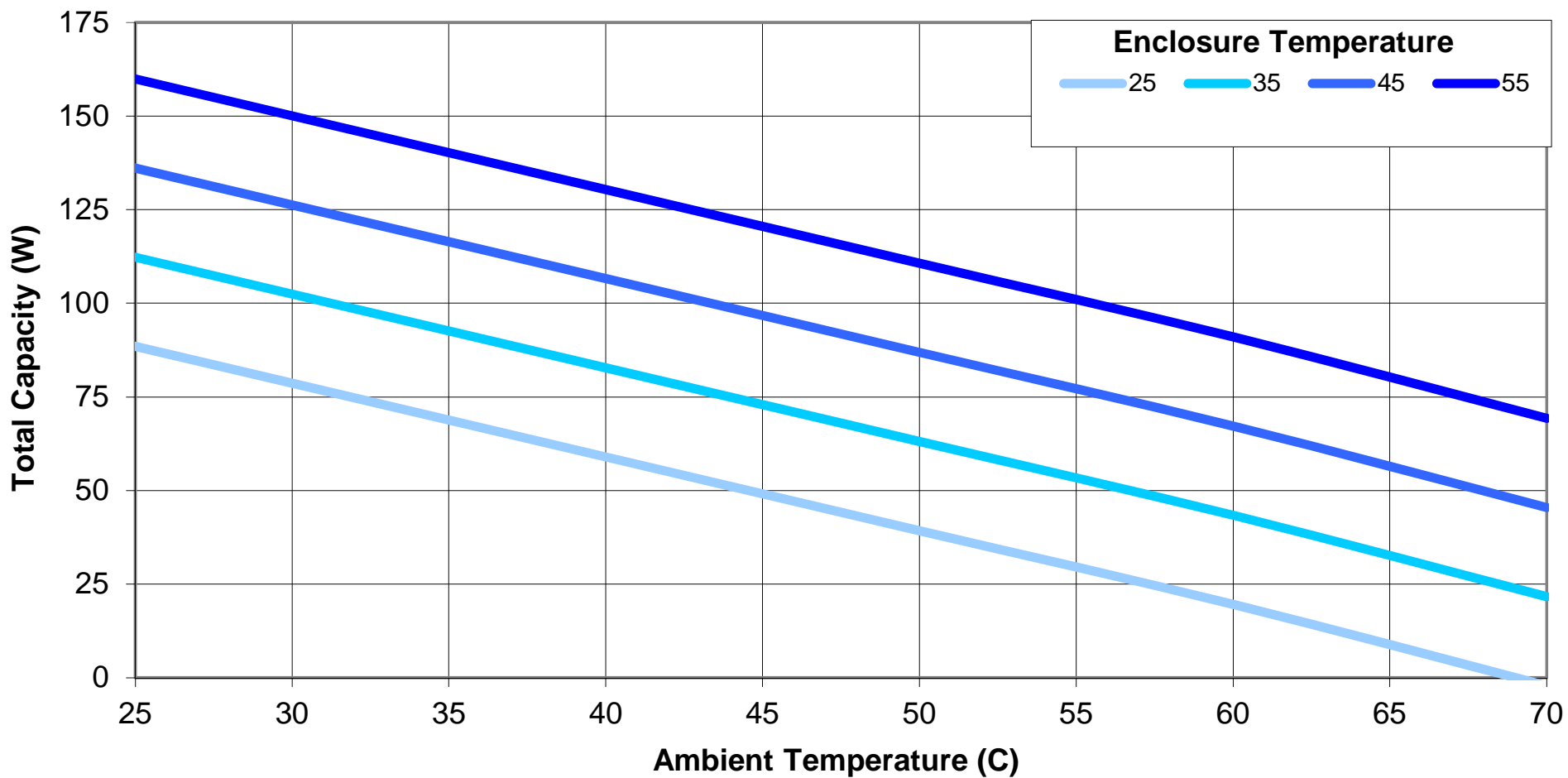
AHP-470 Cooling for various Enclosure Temperatures
