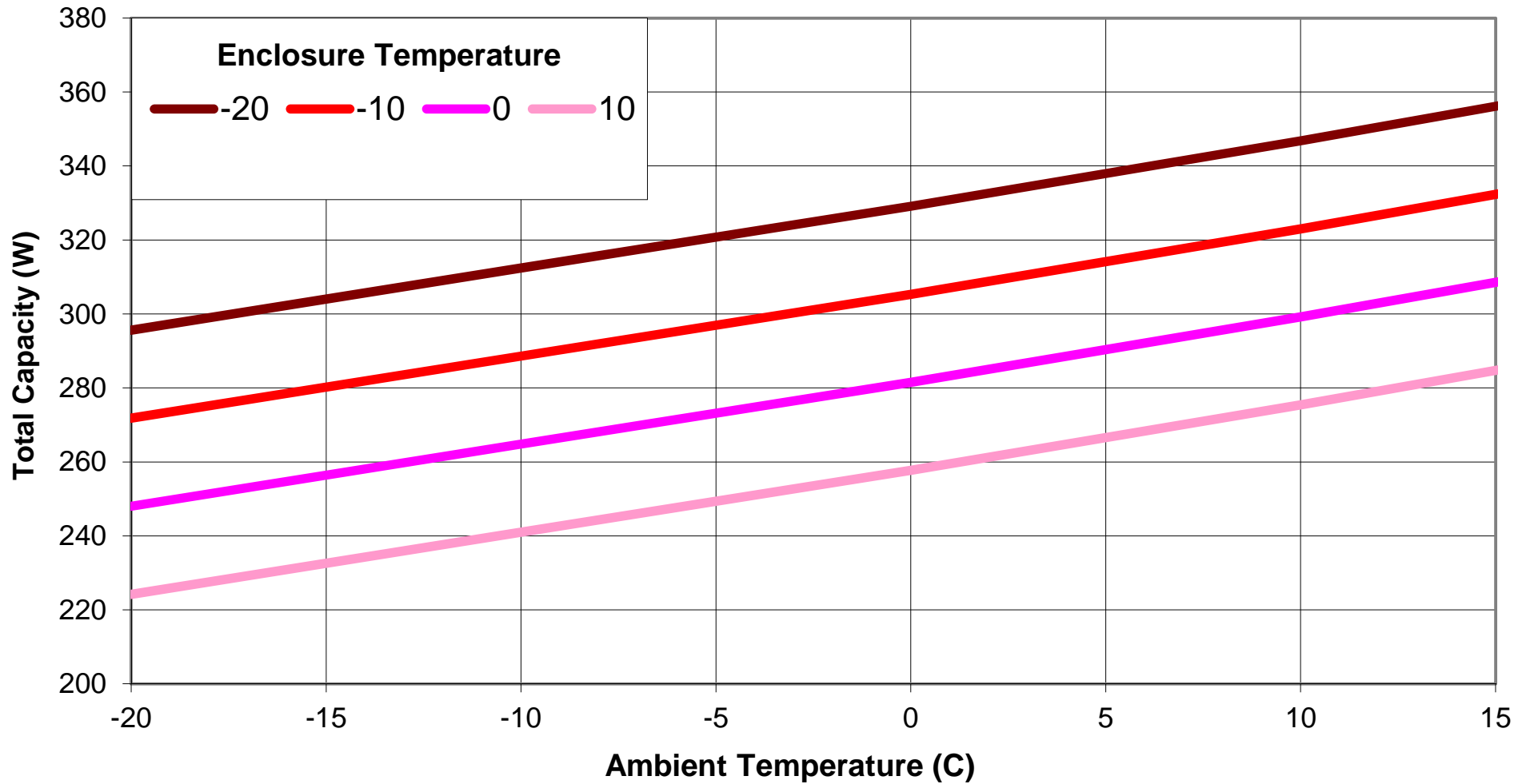
AHP-470 Heat Mode Capacity for various Enclosure Temperatures
