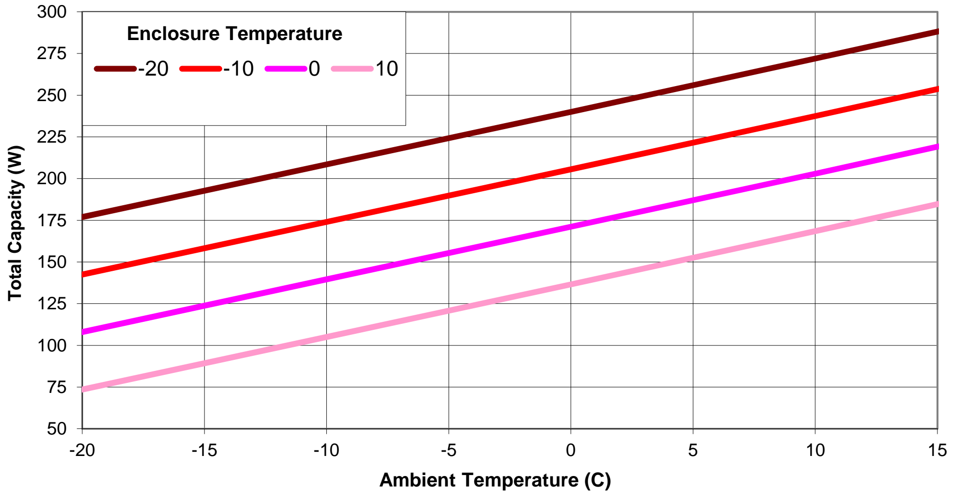
AHP-570 Heat Mode Capacity for various Enclosure Temperatures
