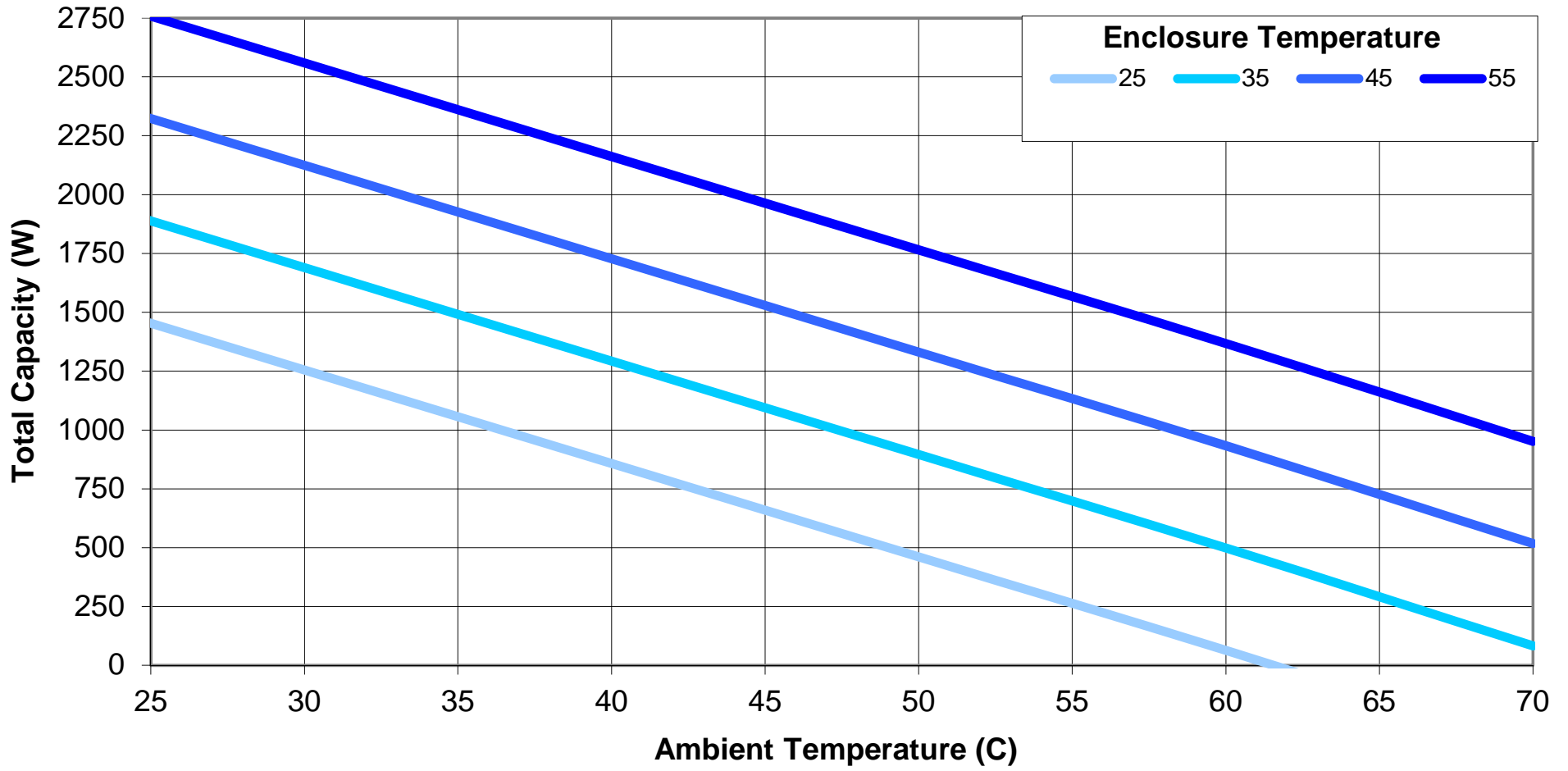
AHP-6253 Cooling for various Enclosure Temperatures
