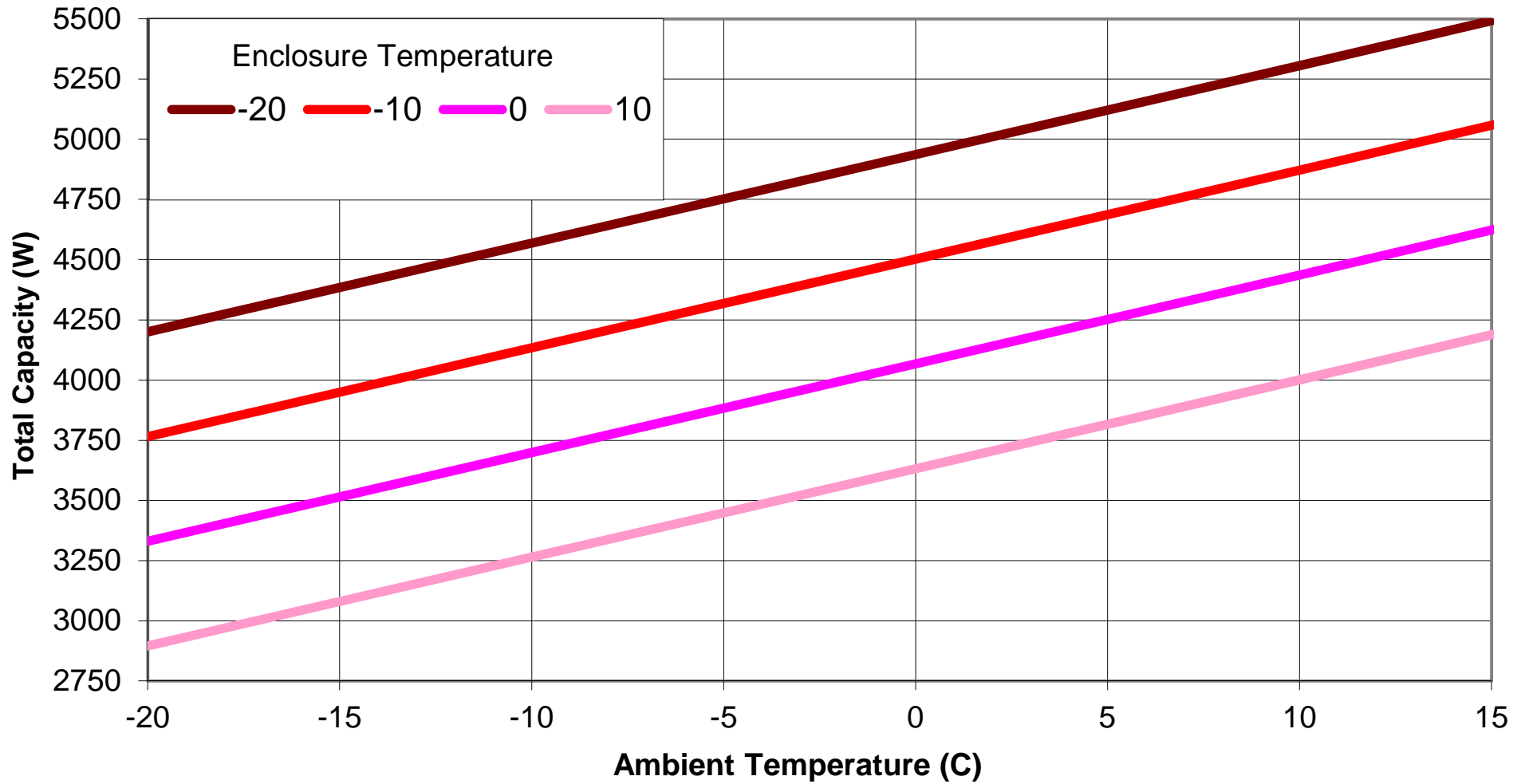
AHP-6253 Heat Mode for various Enclosure Temperatures
