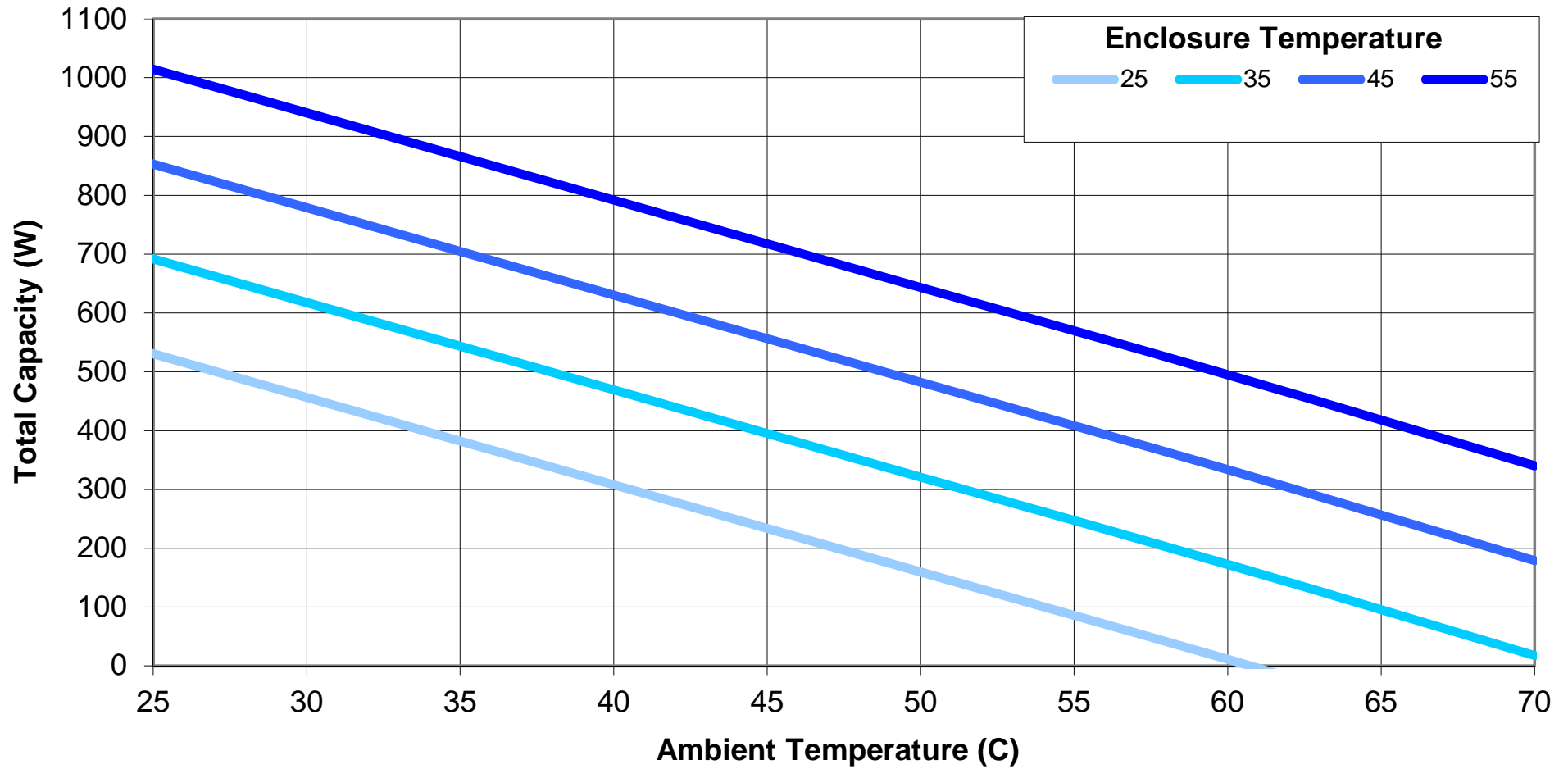
FHP-2250 HiCap Cooling for various Enclosure Temperatures
