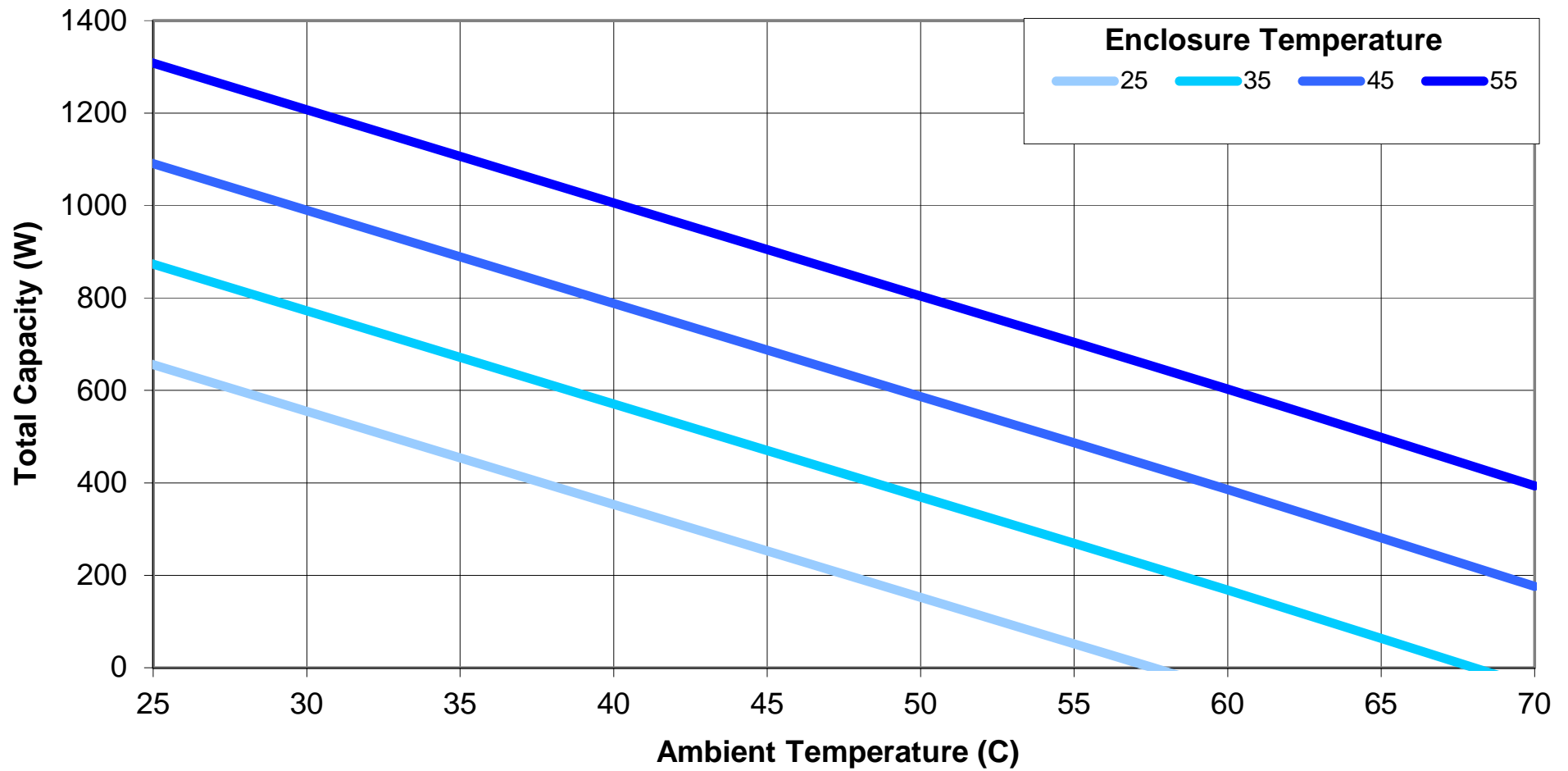
FHP-3252 HiCap Cooling for various Enclosure Temperatures
