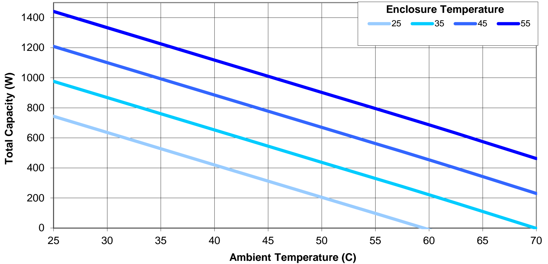
FHP-3253 HiCap Cooling for various Enclosure Temperatures
