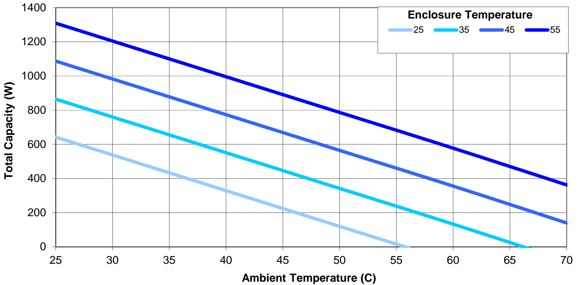
FHP-3254 HiCap Cooling for various Enclosure Temperatures
