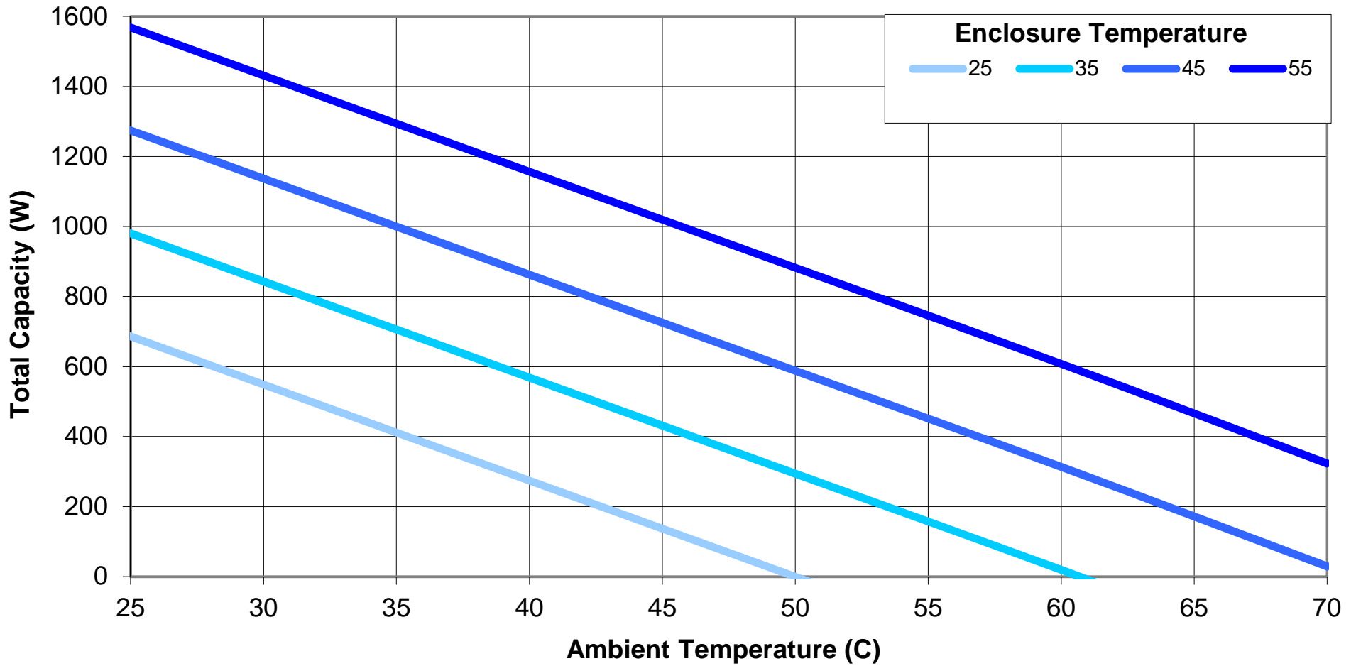
FHP-4250 HiE Cooling for various Enclosure Temperatures
