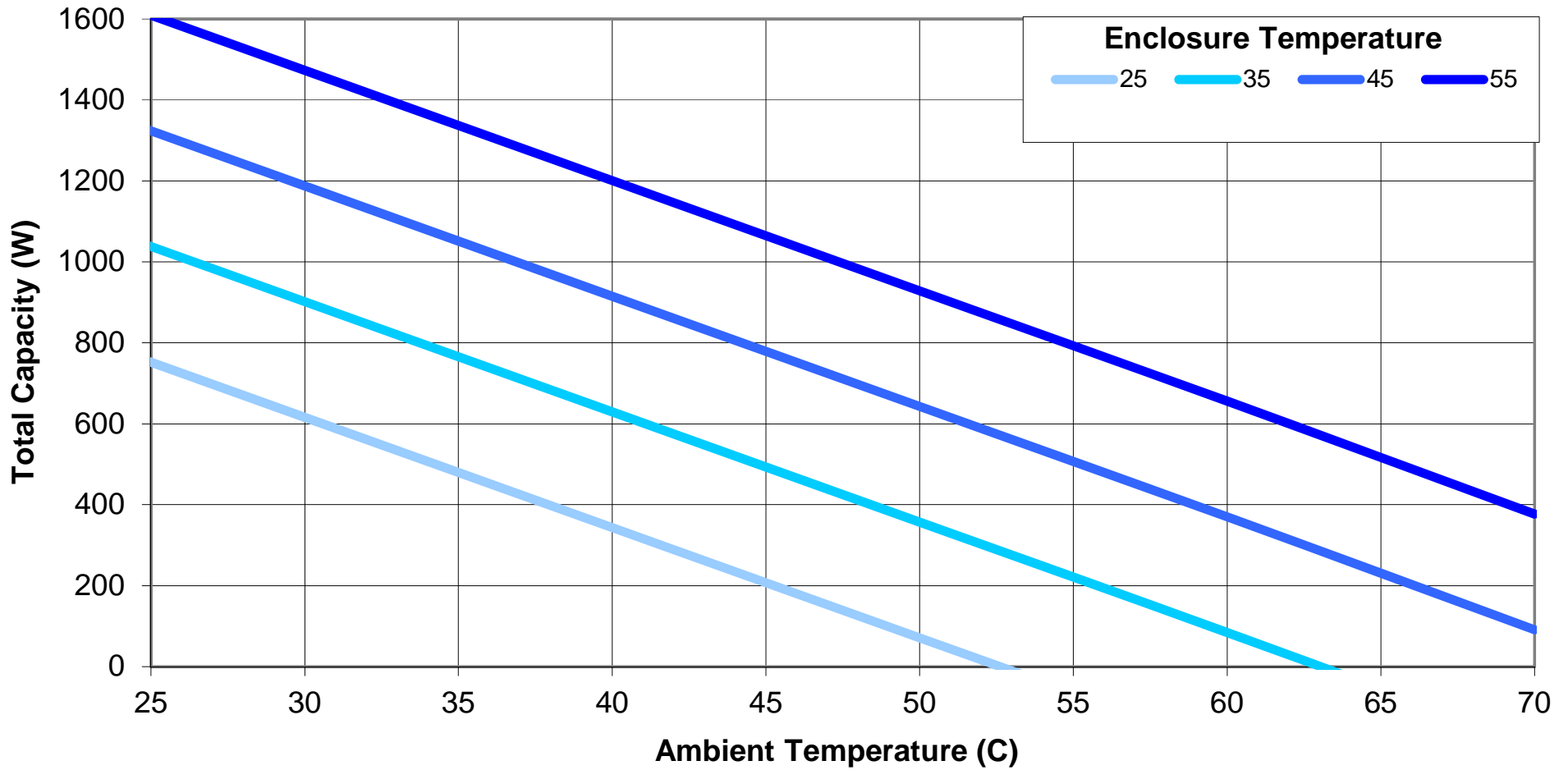
FHP-4252 HiE Cooling for various Enclosure Temperatures
