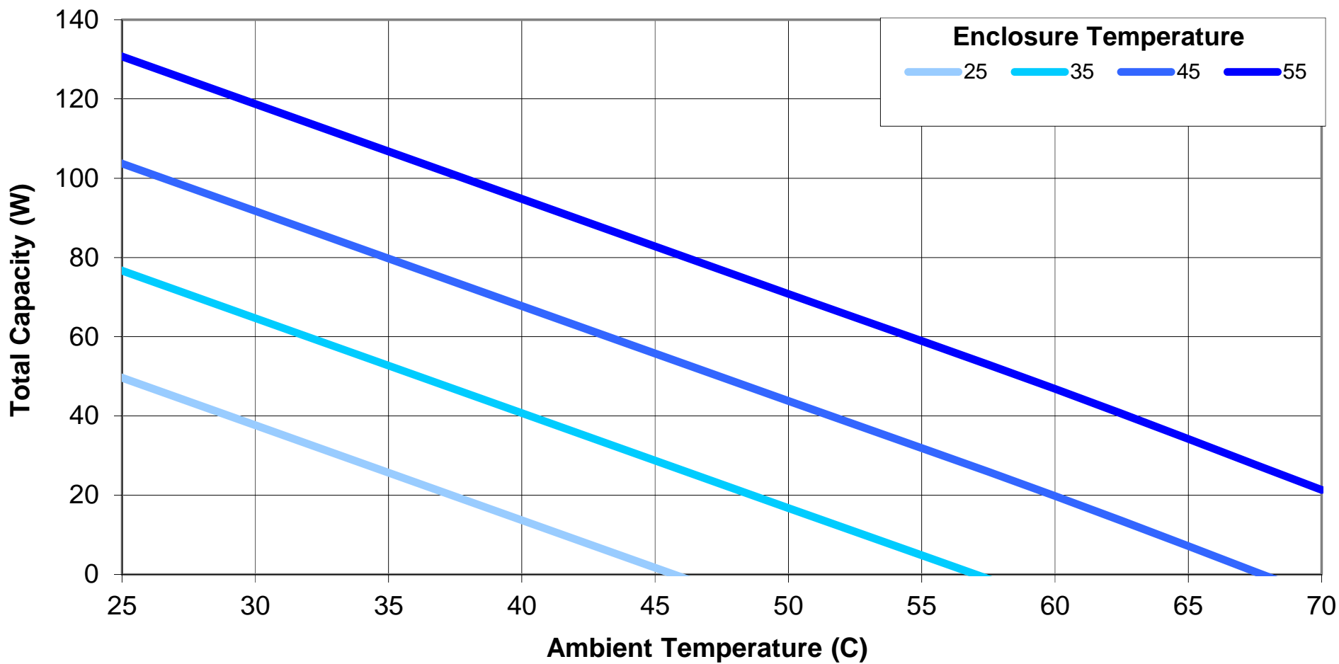
FHP-450 Cooling for various Enclosure Temperatures
