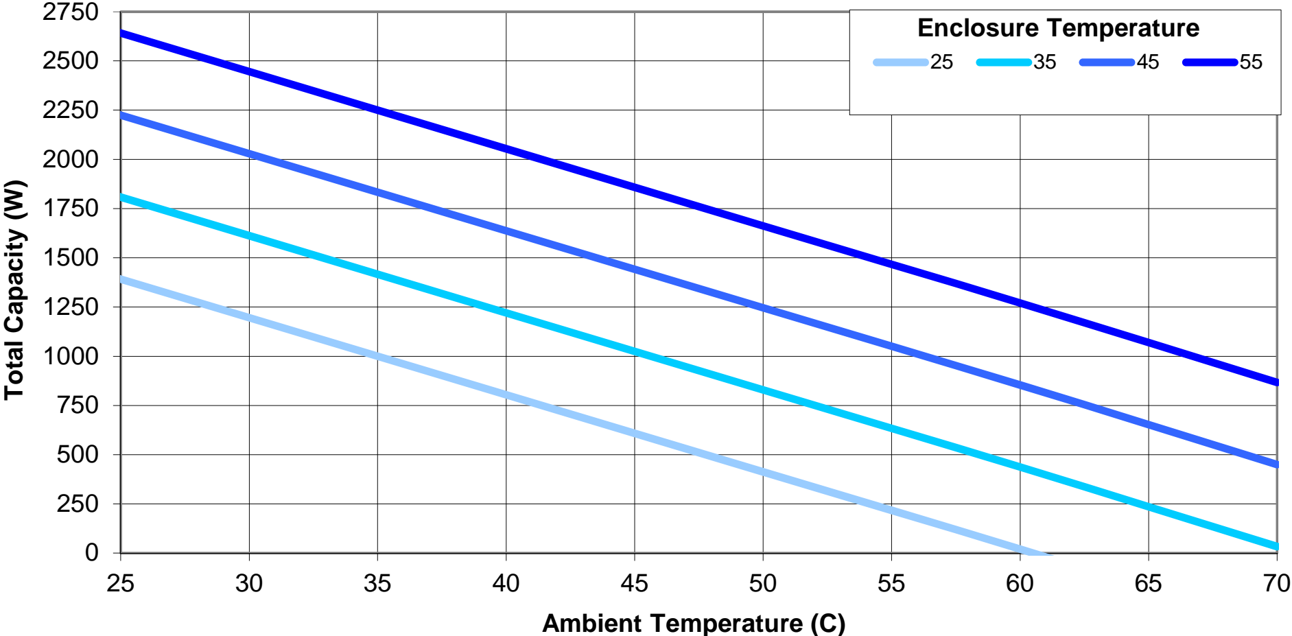
FHP-6253 Cooling for various Enclosure Temperatures
