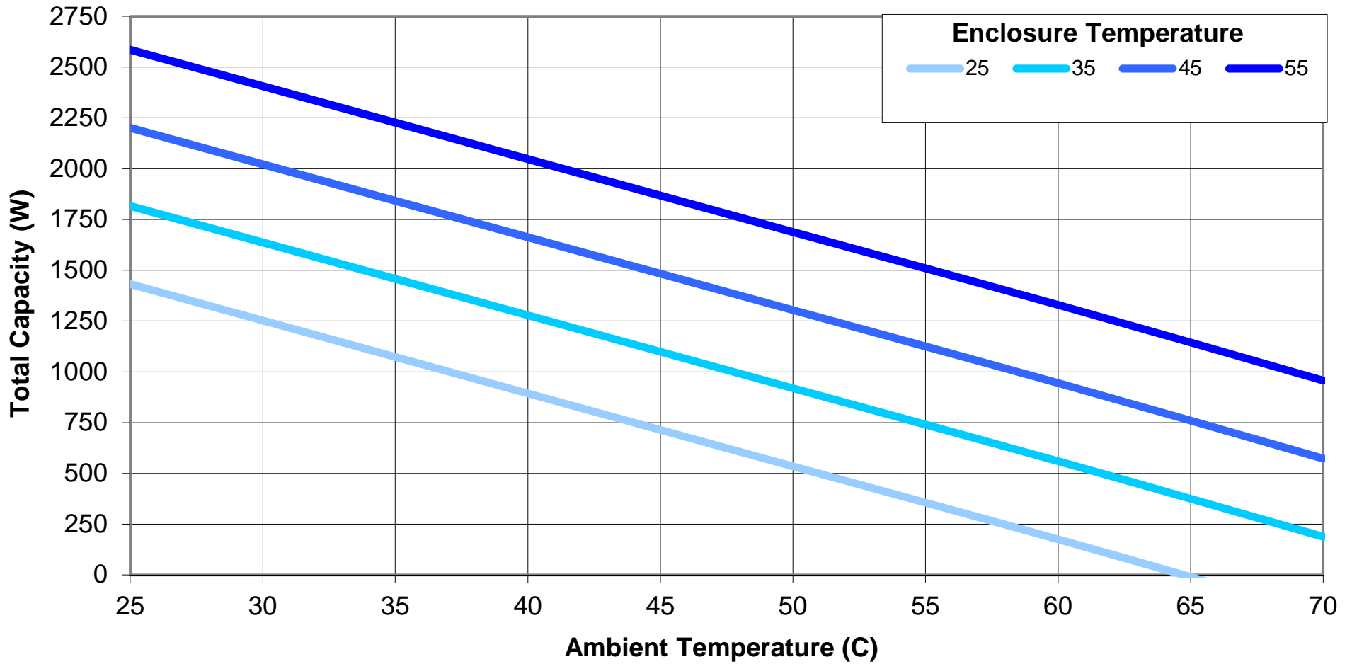
FHP-6263 HiCap Cooling for various Enclosure Temperatures
