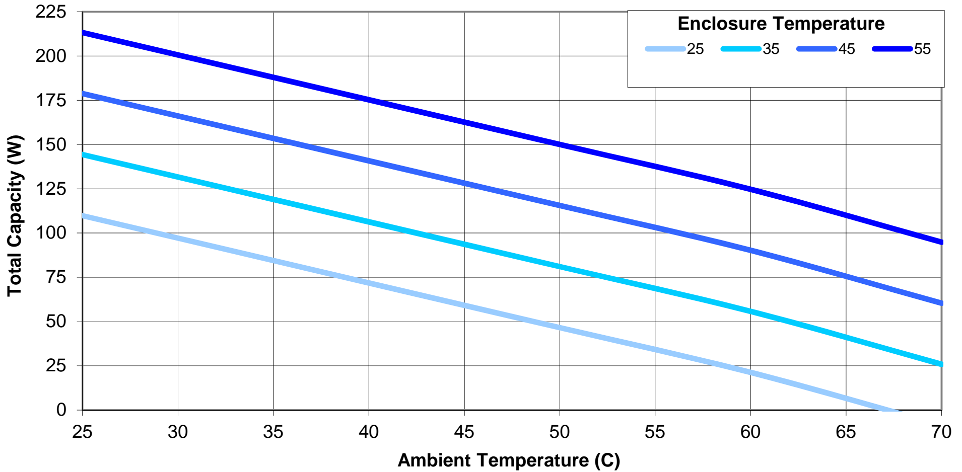
FHP-750 Cooling for various Enclosure Temperatures
