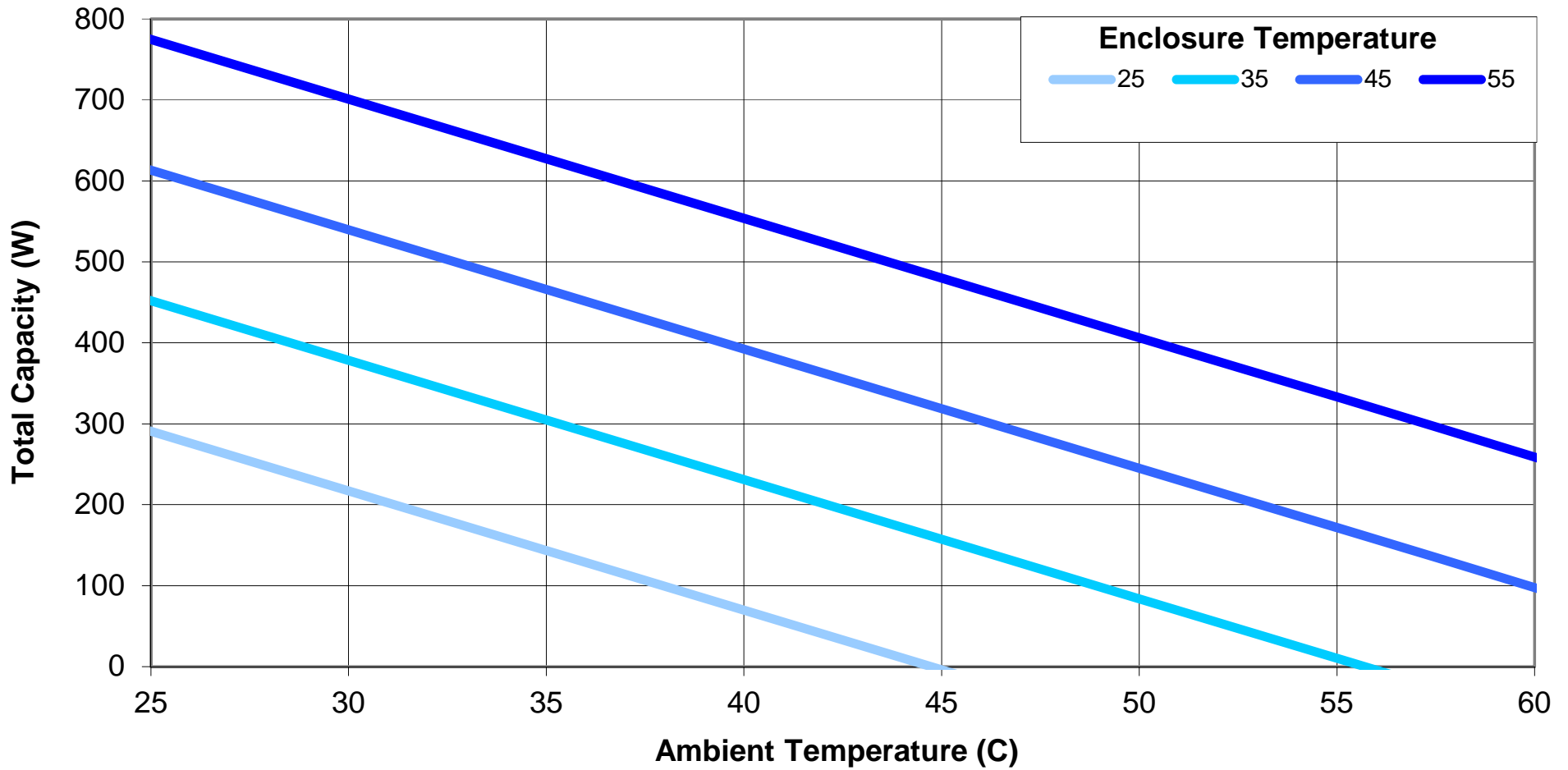
IHP-2259 HiE Cooling for various Enclosure Temperatures
